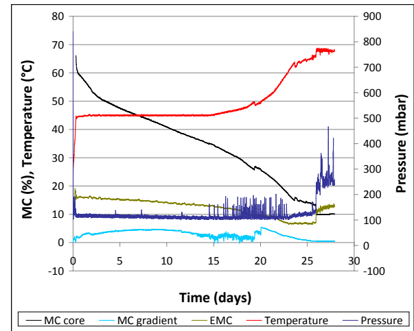
Figure 40. Vacuum drying chart – BBT3 trial
