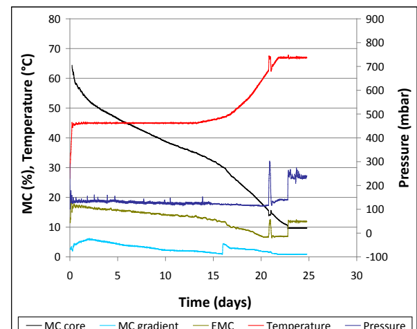
Figure 41. Vacuum drying chart – BBT4 trial
