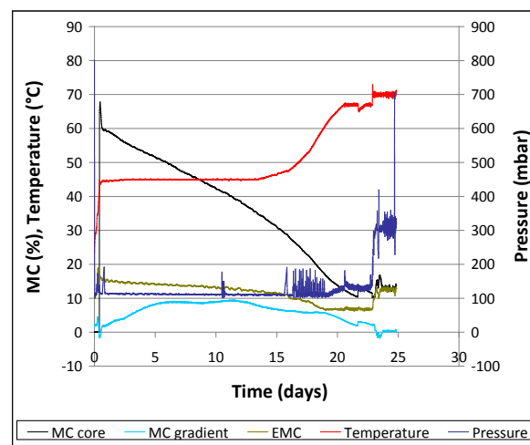
Figure 30. Vacuum drying chart – JAR3 trial
