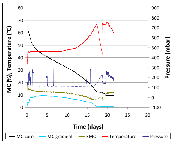
Figure 39. Vacuum drying chart – BBT2 trial
