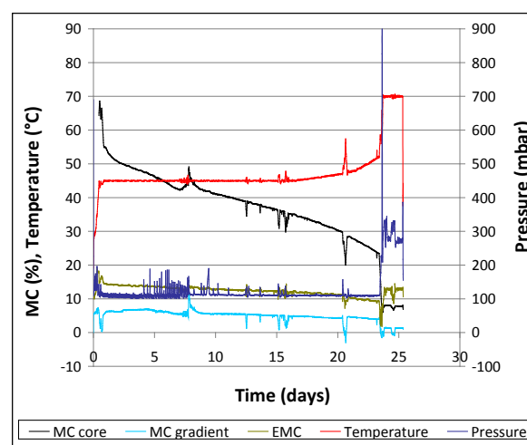
Figure 31. Vacuum drying chart – JAR4 trial
