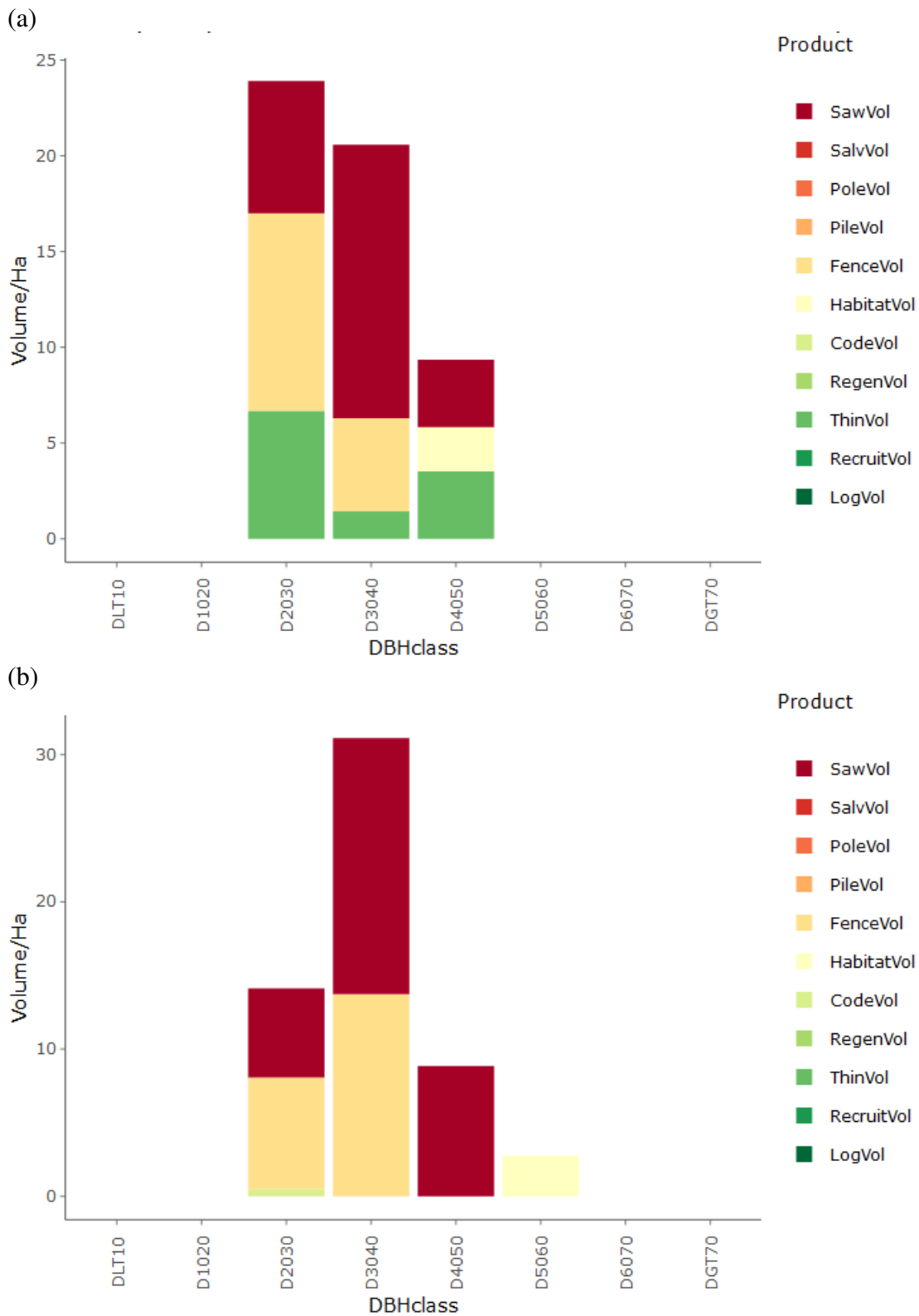
Figure 5.3. Volumes of timber ( m^3/ha ) expected after 20 years in different products and DBH classes. Scenario 1 (a) shows volumes expected where no thinning was applied (the green bars in this case shows the volume in trees that could have been thinned) and Scenario 2 (b) shows volumes were thinning was applied.
