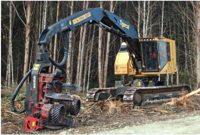
Figure 4: A Tigercat LH22D harvester with Waratah HTH622B harvesting head and a Ponsse Elephant King forwarder were used at the Unpruned Low-Quality (ULQ) and Pruned High-Quality (PHQ) sites.
