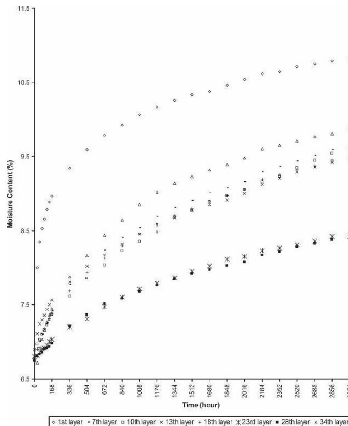
Figure 28: MC change by layer. (Zhang et al., 2006)
