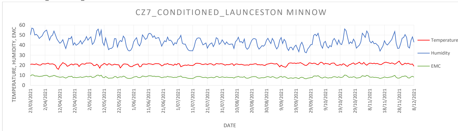
Figure 1. Temperature, Humidity, and calculated EMC
