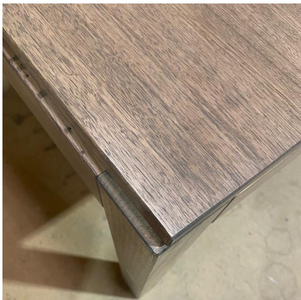
Figure 8: Shrinkage along a tabletop leading to an exposed rail edge
