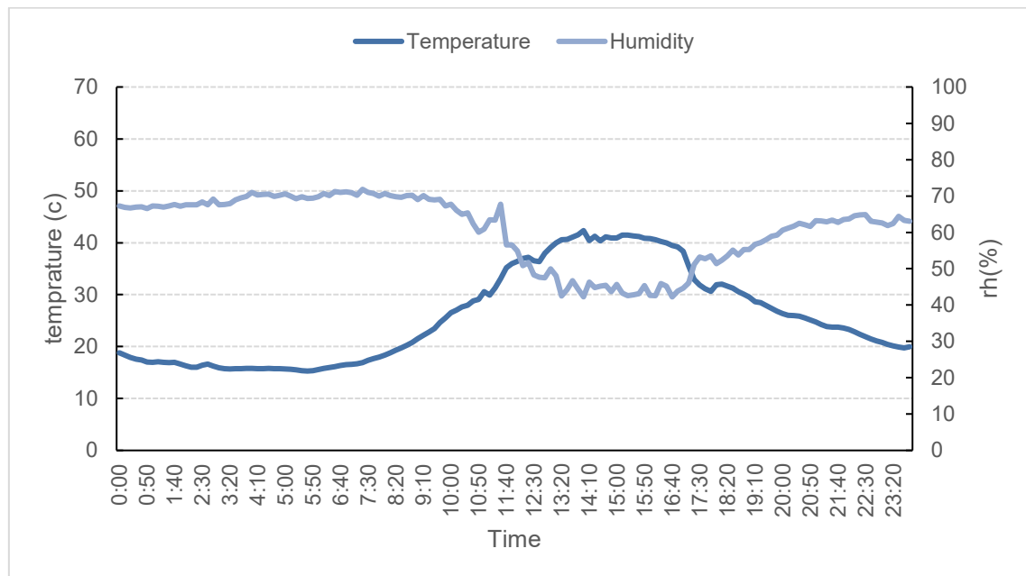
Figure 11 Measured environmental conditions in an exterior poorly wrapped CZ7 pack on January 15, 2022. Sensor - north facing top middle
