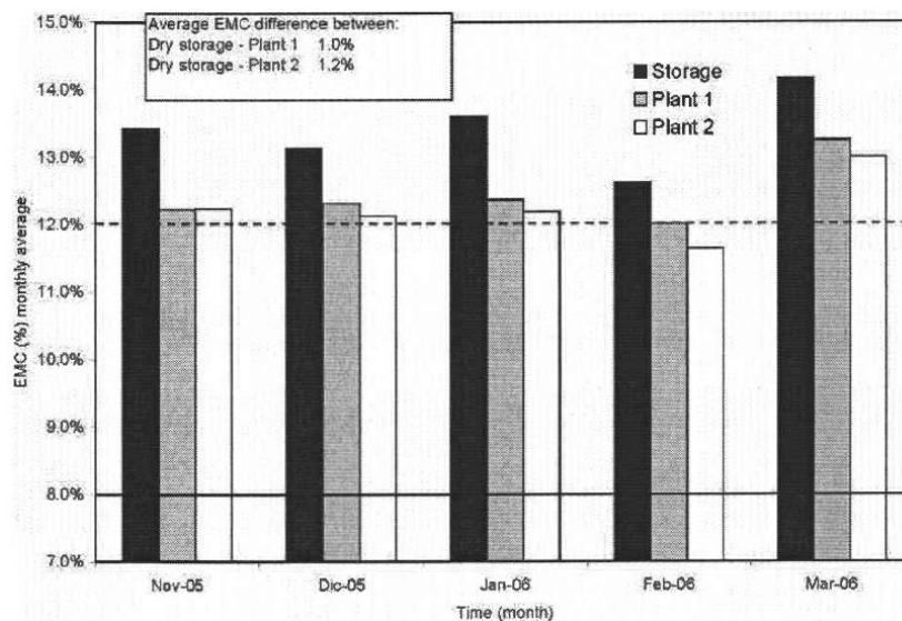
Figure 32: Monthly average EMC values for plant (three-walled shed configuration) in Santa Cruz-Bolivia. November 2005 to March 2006. Continuous and dashed horizontal lines represent respectively, lumber MC after drying for millwork (8%) and garden furniture (12%).
