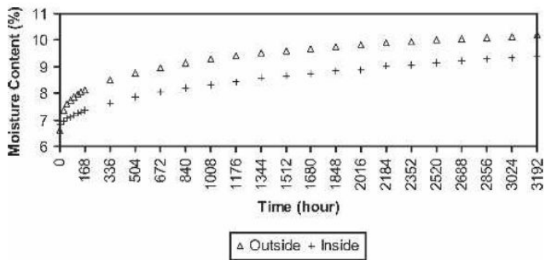
Figure 30: MC comparison between outside and inside boards.
