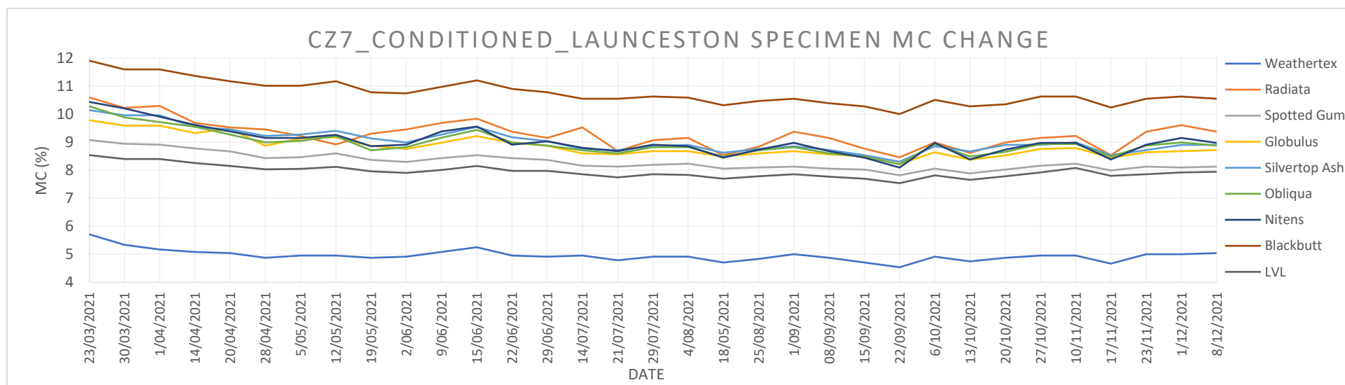
Figure 2. Change in MC for static timber specimens
