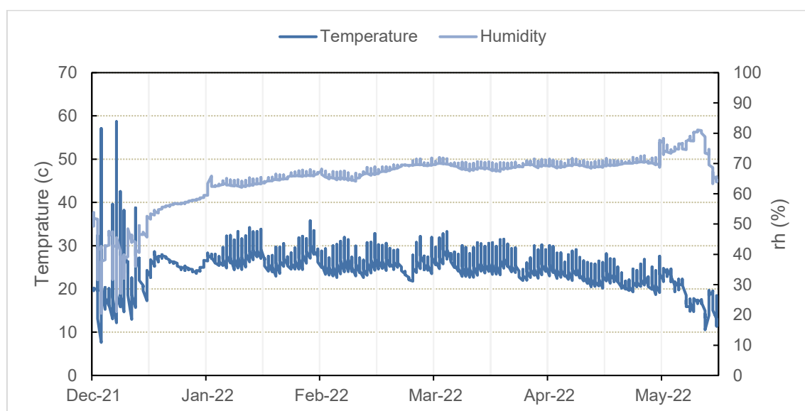
Figure 44 Measured environmental conditions in a CZ2 pack. Sensor - north facing top middle
