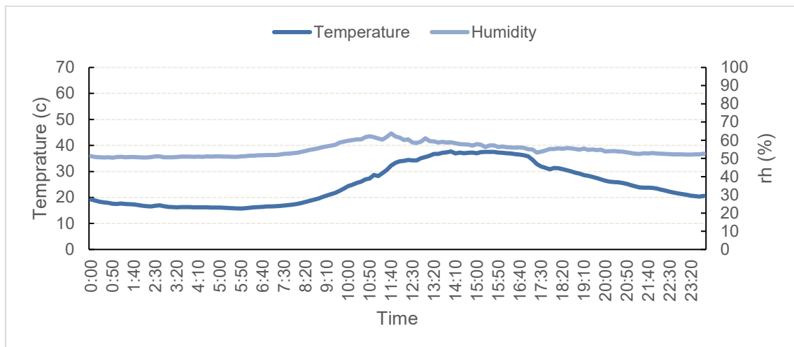
Figure 19 Measured environmental conditions in an exterior fully wrapped - opaque CZ7 pack on January 15, 2022. Sensor - north facing top middle
