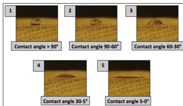
Figure 23. Examples of water droplet shapes on timber that were used to quantify water repellence of the treated and untreated Eucalyptus timbers (Photo: Greeley Beck, Oregon State University).
