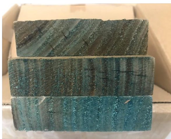
Figure 31. Cross sections of three oven-dried 25 mm thick shining gum samples after 10 wet/dry cycles showing minor internal splits. Photo: Jeffrey Morrell.
