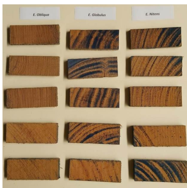
Figure 16. E. obliqua , E. globulus , E. nitens , (left to right) Charge 2 (matching boards in Figure 15 above) board cross sections treated with ACQ and sprayed with chrome azurol S, showing less penetration than with PAN indicator spray. Photo: Stuart Meldrum.
