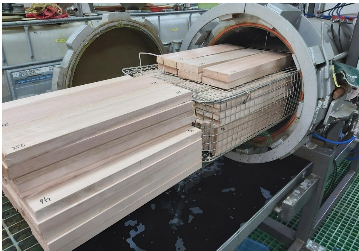
Figure 14. Untreated boards in preparation for VPI treatment in cylinder at DAF. Photo: Stuart Meldrum.
