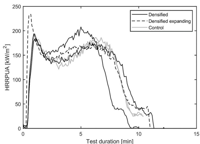
Figure 35. Heat release rates for densified and non-densified shining gum samples during cone-calorimeter testing.
