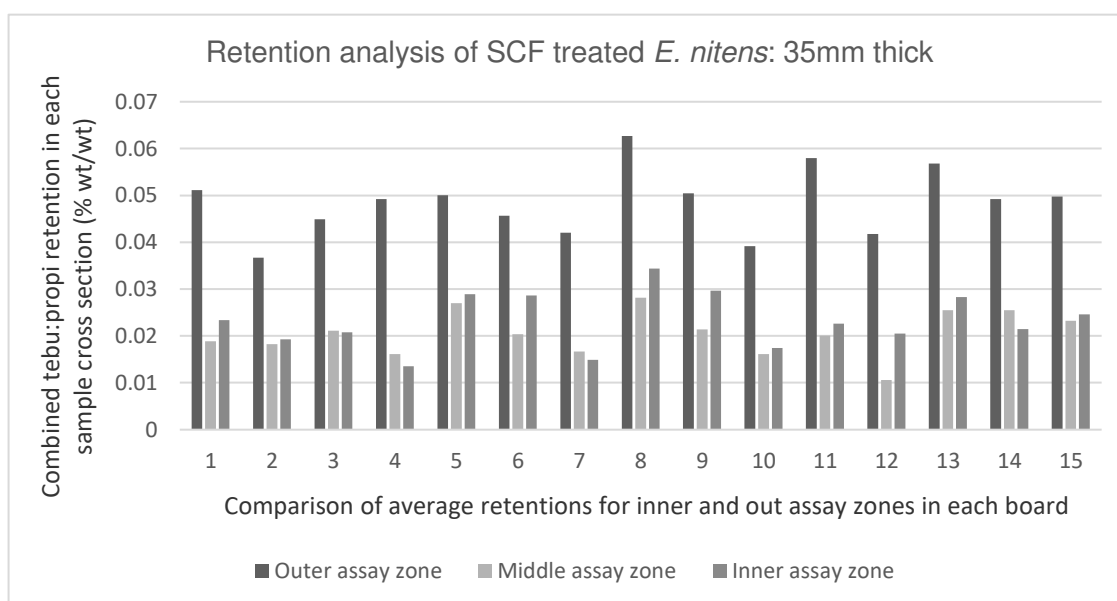
Figure 22. Retention of tebuconazole/propiconazole at selected depths in 35mm thick shining gum boards treated using supercritical carbon dioxide.
