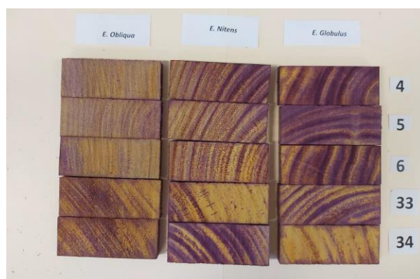
Figure 15. E. obliqua , E. nitens , E. globulus (left to right) Charge 2 board cross sections treated with ACQ and sprayed with PAN indicator showing reasonable penetration, particularly in back sawn E. globulus . Photo: Stuart Meldrum.
