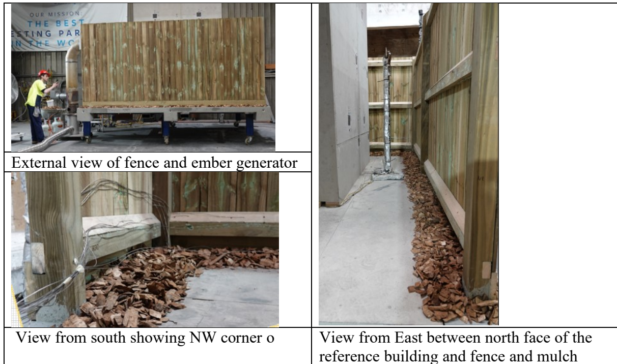
Figure 55 General Arrangement of test 1 paling fence before test
