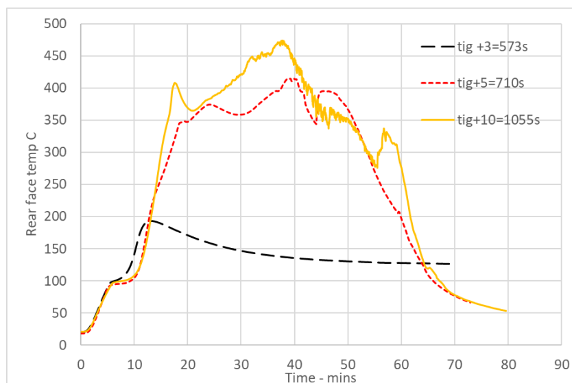
Figure 23 Rear face temperatures for 12mm thick treated radiata pine subjected to an irradiance of 19\text{kW/m}^2 -black long dashes show specimen with heating terminated 3 minutes after flaming ignition (total exposure 573s) which self-extinguished when heat source removed. Red and yellow plots show specimens with longer exposures that continued smouldering combustion until the timber was effectively consumed
