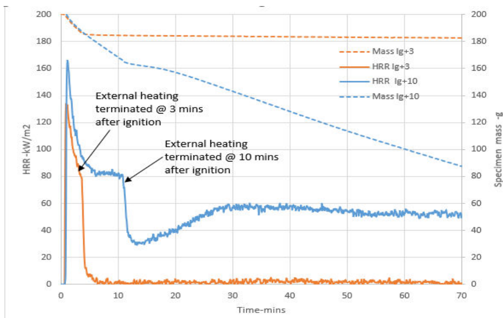
Figure 26 HRR and mass for 45mm thick treated radiata pine subjected to an irradiance of 29\text{kW/m}^2 after conditioning at 30^\circ\text{C}/25\% r.h.- blue plots show specimen with heating terminated 10 minutes after flaming ignition (total exposure 653s) exhibiting sustained smouldering combustion behaviour; brown plots show specimen with heating terminated 3 minutes after flaming ignition (total exposure 222s) exhibiting self-extinguishment behaviour.
