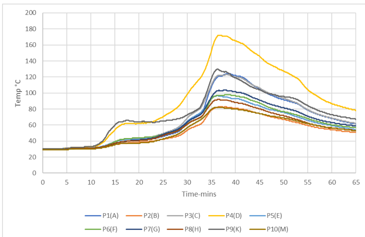
Figure 66 Plate thermometer measurements on the north face of simulated building
