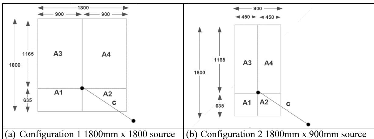
Figure 68 Assumed heat sources for checking separation distances.
