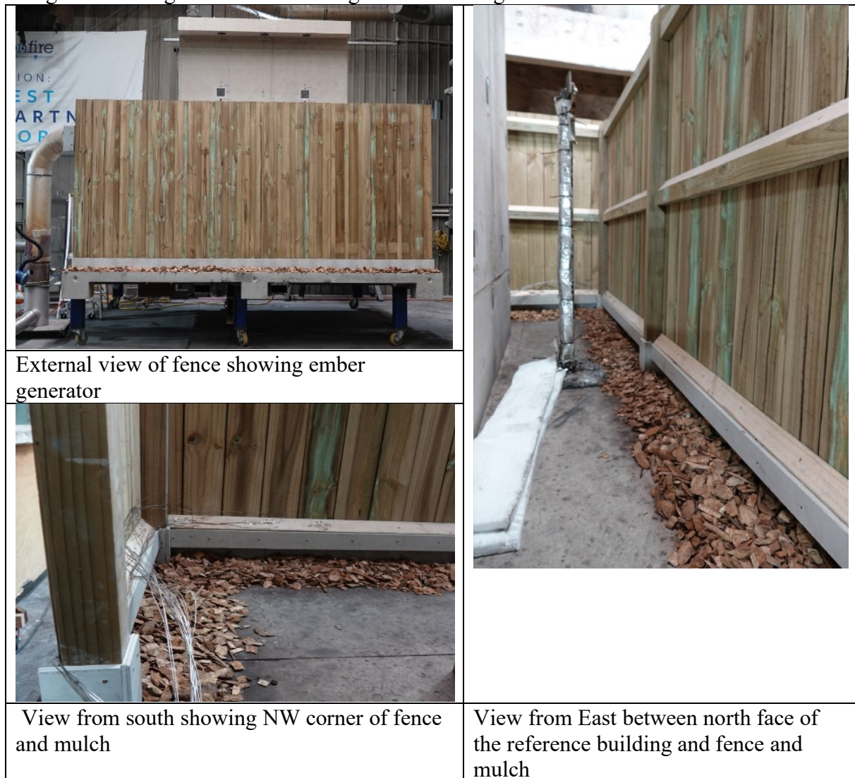
Figure 69 General Arrangement of test 2 paling fence before test with additional protection at base
