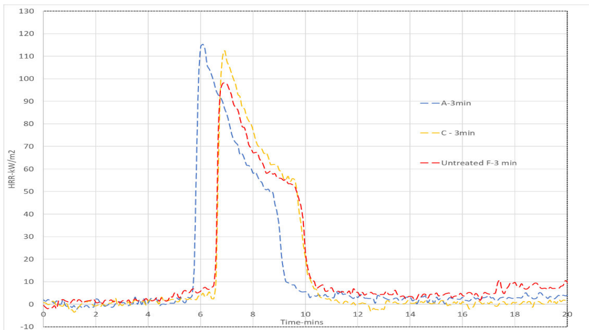
Figure 8 Heat Release Rate for 12mm palings with treatments A and C and untreated exposed to an irradiance of 19\text{kW/m}^2 before ignition and a further 3 minutes
