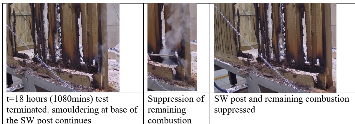
Figure 42 Termination of test 2
