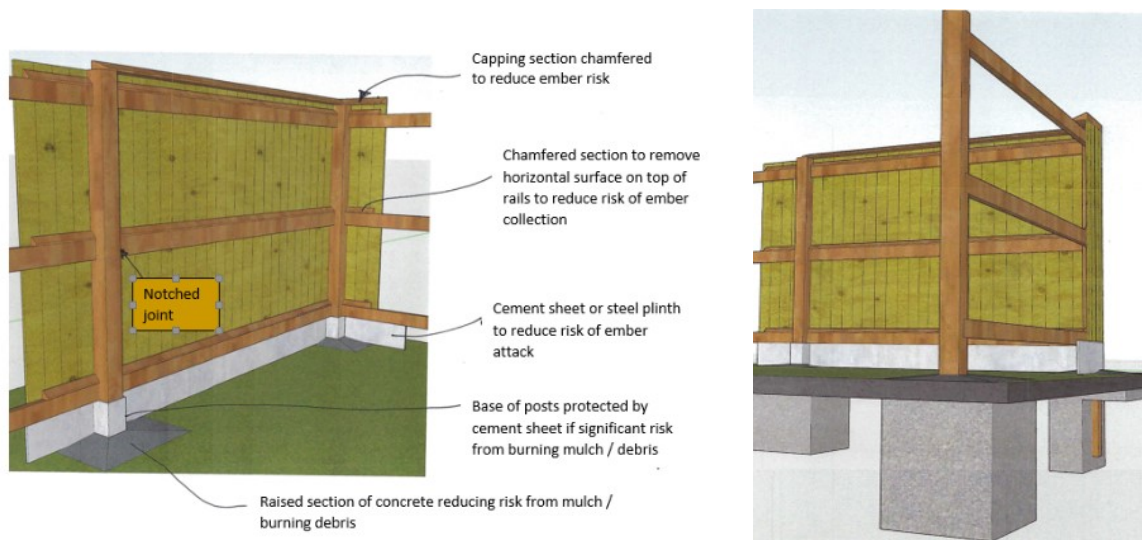
Figure 8 Paling fence designed to shed embers and resist ignition by collections of burning debris at the base of the fence
