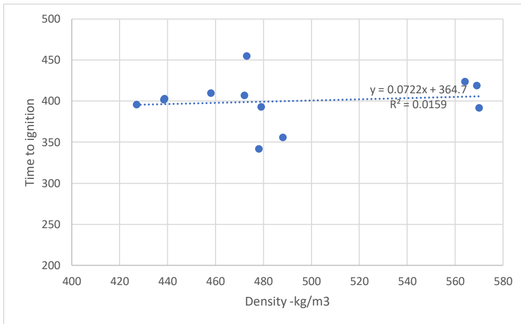
Figure 17 Time to ignition against density for 12mm paling samples at an irradiance of 19kW/m 2
