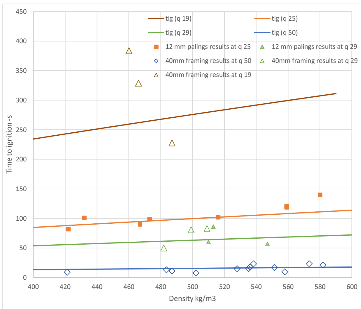
Figure 19 Comparison of Babrauskas correlation with density and typical results from Stages 1 and 2
