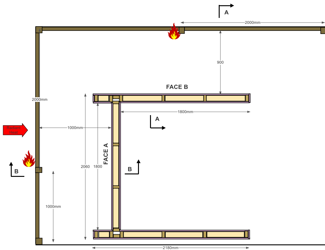
Figure 17 Fence facing bushfire hazard 1m from face of reference building with return running perpendicular to bushfire hazard 900mm from the building
