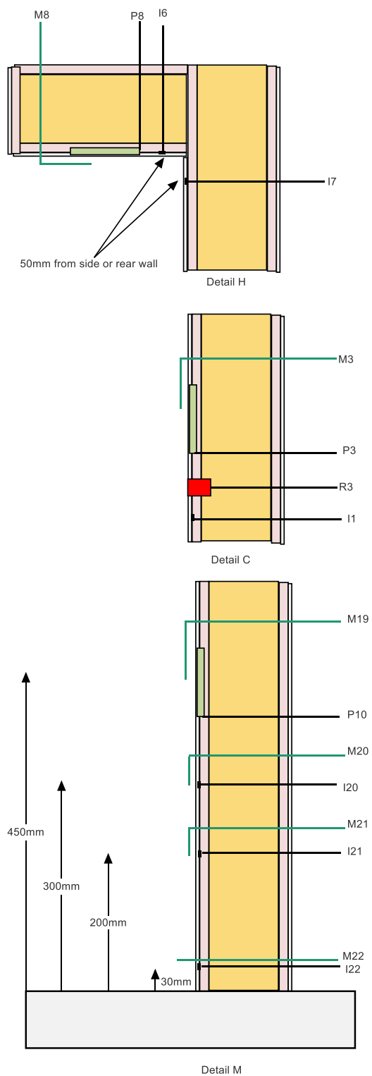
Figure 26 Section showing typical instrumentation details for the west face
