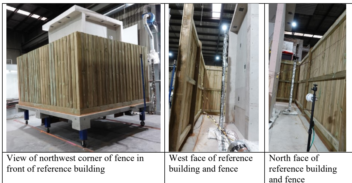
Figure 29 Test 1 Fence and reference building before test
