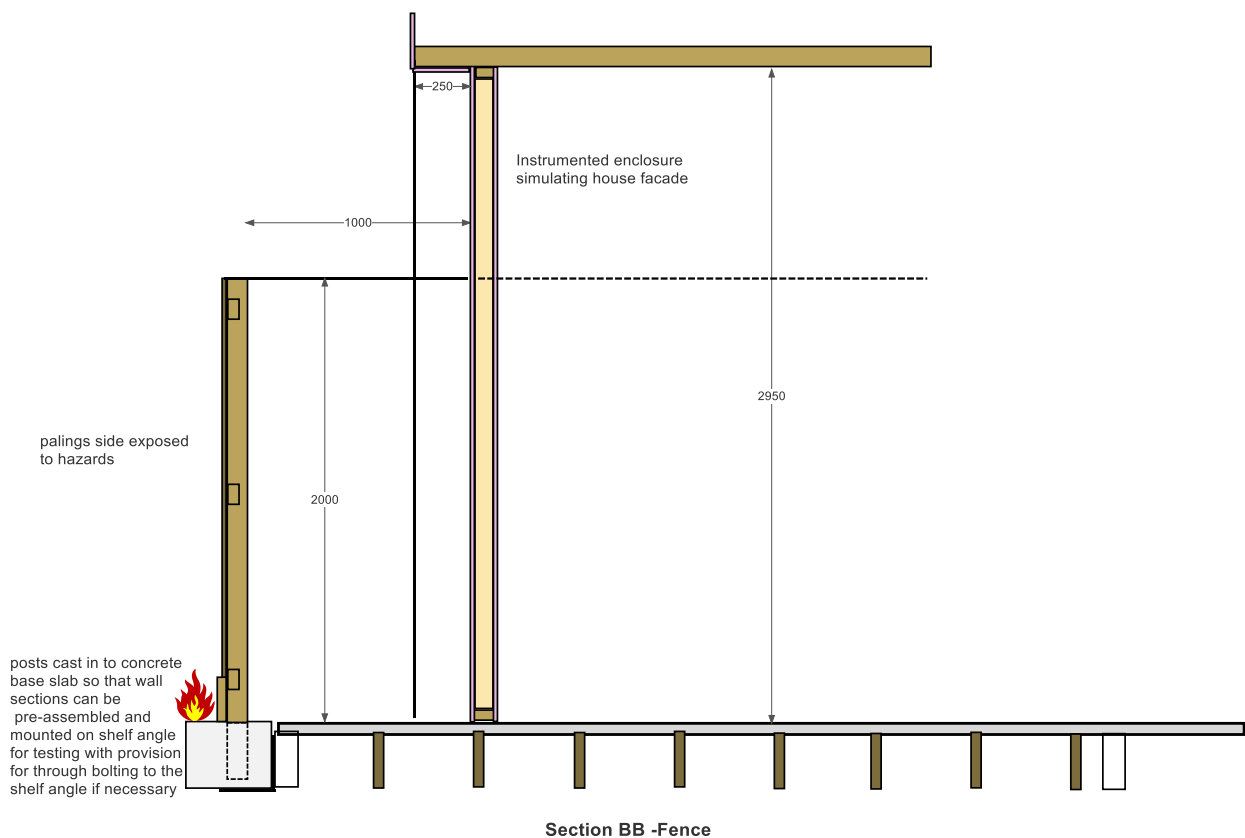
Figure 18 Longitudinal section B-B through fencing and reference building
