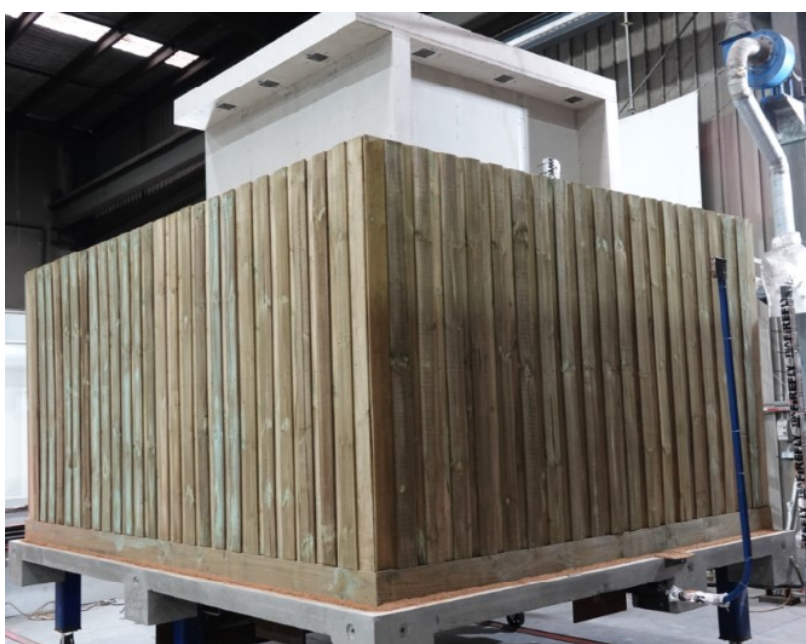
Figure 16 General view of test configuration for fencing tests
