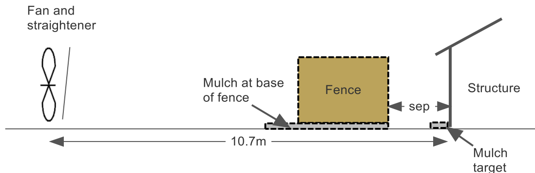
Figure 52 Typical test configuration for wind-driven fire spread to a structure from fences and mulch used in Nist experiments by (Butler, Johnsson et al. 2022)
