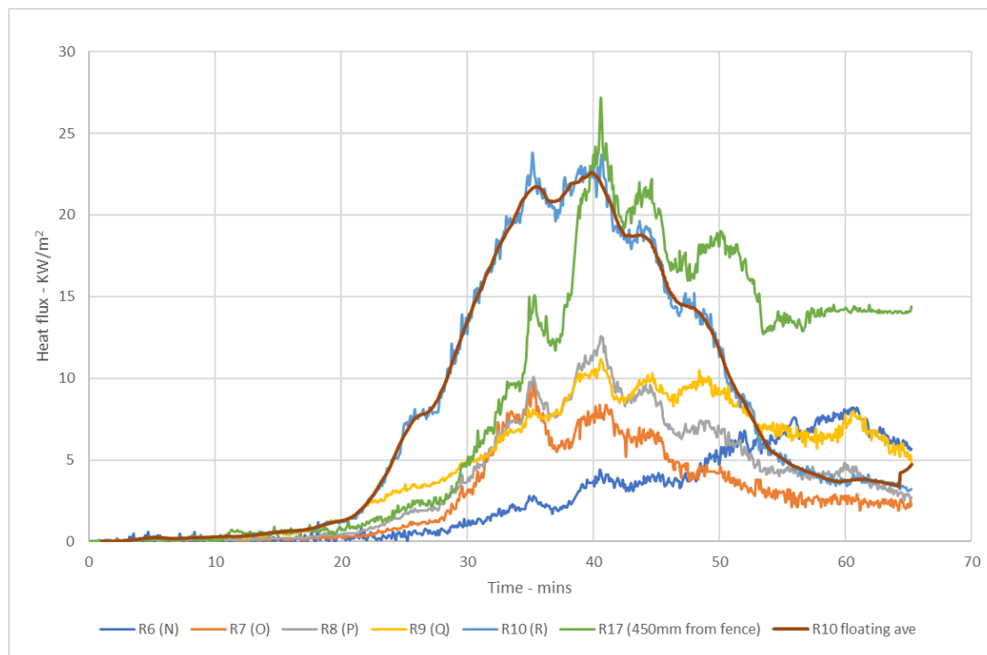
Figure 63 Ember test 1 Heatflux measured on north face of structure and 450mm from fence
