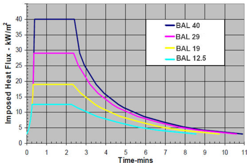
Figure 12 AS1530.8.1 Radiant Heat Profiles based on AS 1530.8.1
