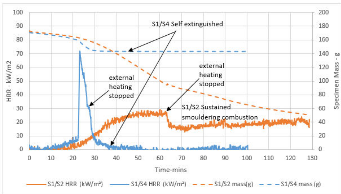
Figure 24 HRR and specimen mass for 45mm thick treated radiata pine subjected to an irradiance of 12.5\text{kW/m}^2 - blue plots show specimen with heating terminated 5 minutes after flaming ignition (total exposure 27.75mins); Brown plots show specimen that underwent smouldering ignition only with heating continued for total exposure of 63 minutes
