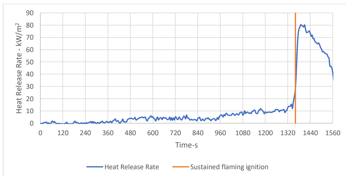
Figure 14 HRR for treated pine (preservative C) 39mm thick exposed to an Irradiance of 12.5\text{kW/m}^2
