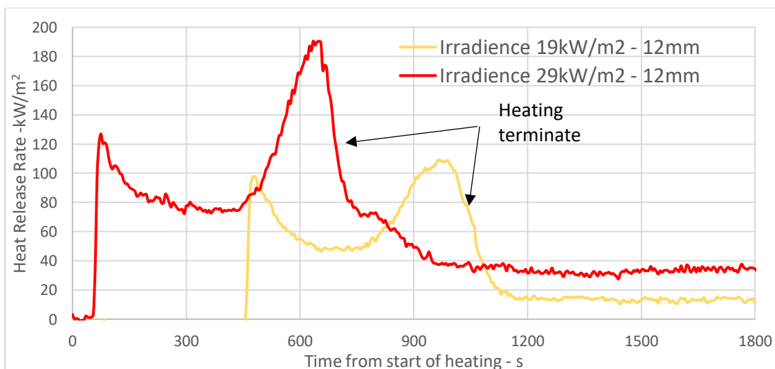
Figure 31 HRR from fire cone calorimeter tests on radiata pine, nominally 12 mm thick with preservative treatment C at varying irradiances for a heating duration of 600s after ignition – specimens conditioned at 23°C and 50% relative humidity.
