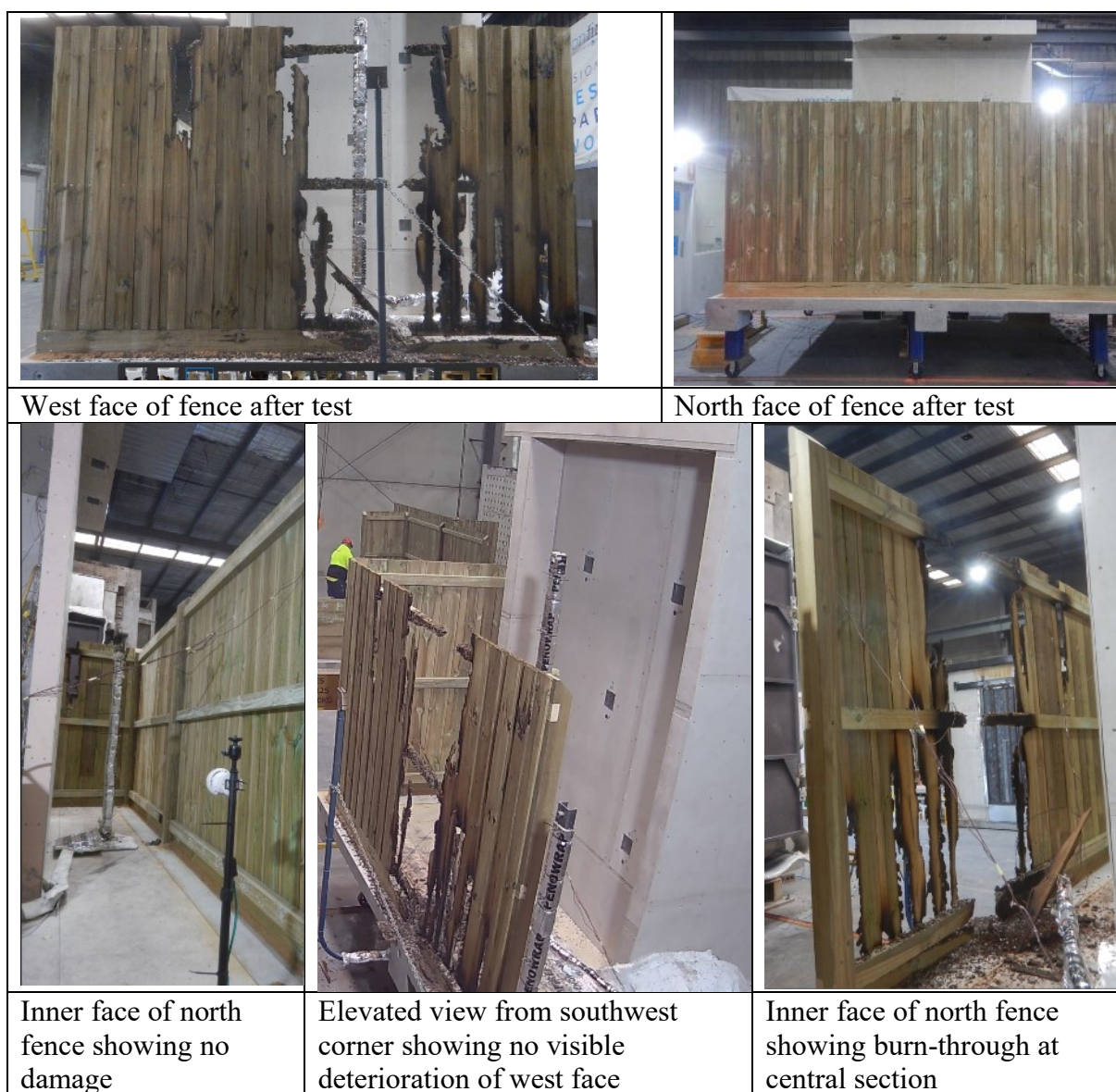
Figure 43 View of specimen after test.
