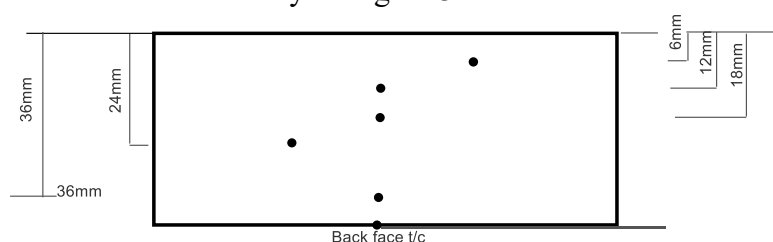
Figure 32 Internal thermocouple measurement positions for timber paling / framing cone calorimeter samples
