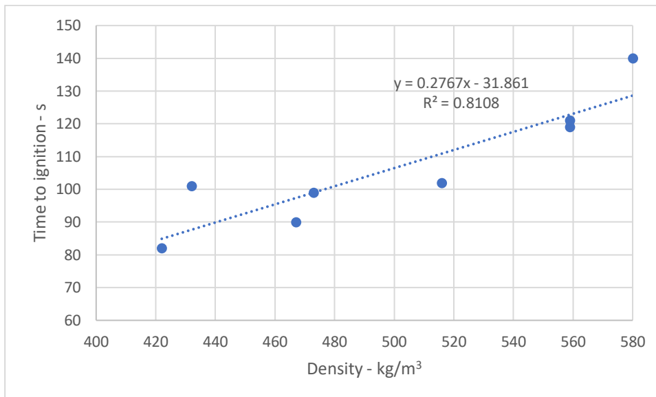
Figure 18 Time to ignition against density for 12mm paling samples at an irradiance of 25kW/m 2
