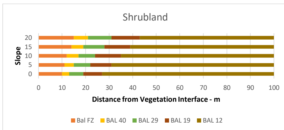
Figure 6 AS 3959 2009 BAL Levels v Distance from Shrubland for varying Downslopes for an FFDI of 100 using the Simple Method Tabulated Values
