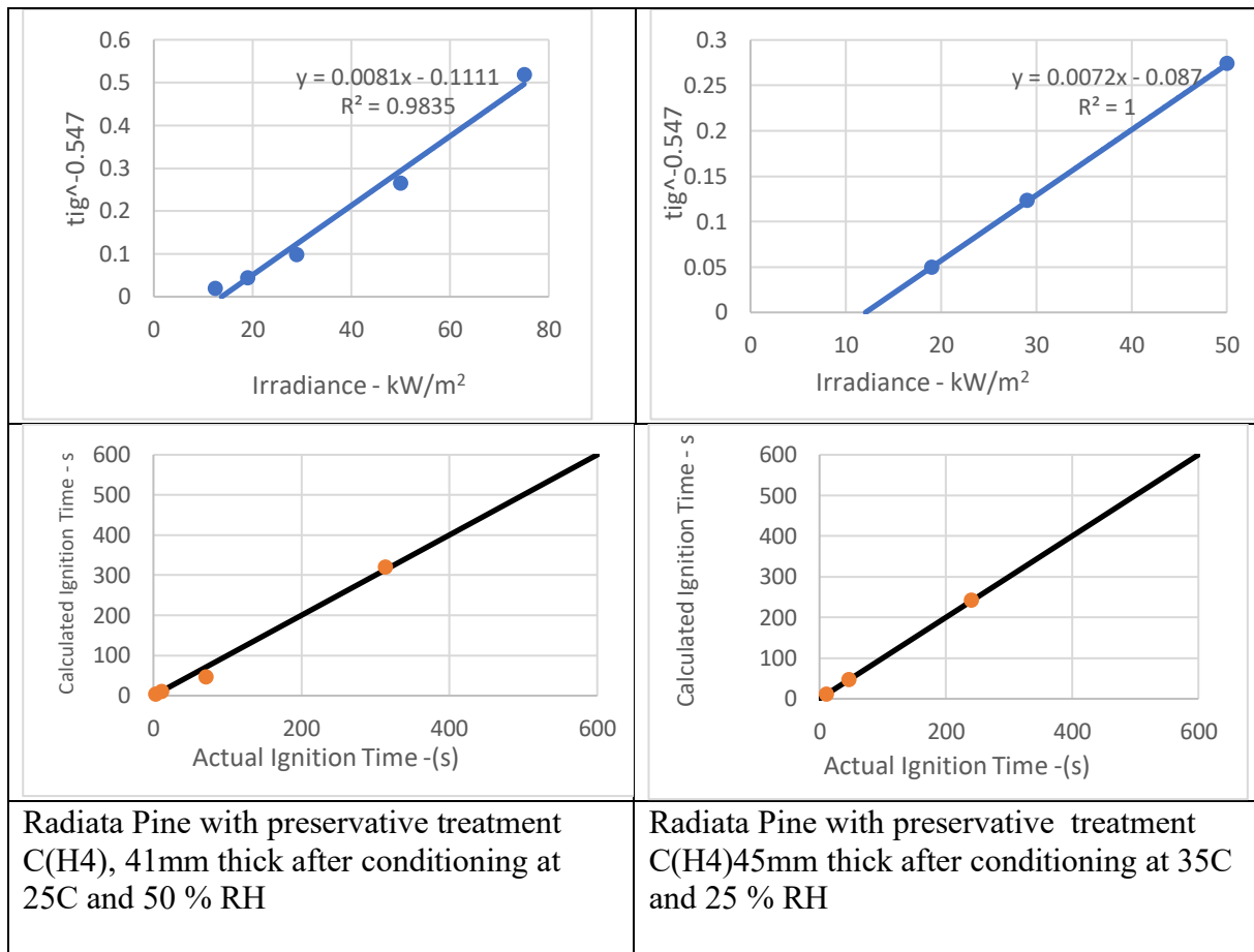
Figure 15 Application of Janssens method for determination of time to ignition for thick specimens of Radiata Pine with preservative treatment C(H4)
