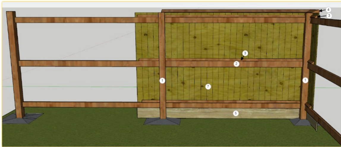
Figure 5 Paling fence viewed from house side. Note components 3 and 4 are not used for the basic system.
