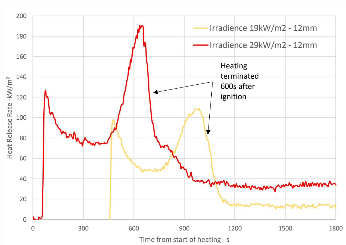
Figure 21 HRR from fire cone calorimeter tests on radiata pine, nominally 12 mm thick with preservative treatment C at varying irradiances for a heating duration of 600s after ignition – specimens conditioned at 23°C and 50% relative humidity.
