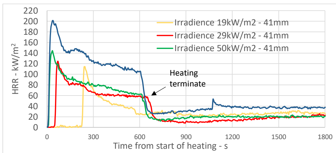
Figure 11 HRR from fire cone calorimeter tests on radiata pine, nominally 41mm thick with preservative treatment C at varying irradiances for a heating duration of 600s after ignition – specimens conditioned at 23°C and 50% relative humidity.
