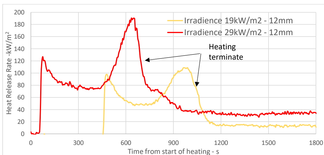
Figure 12 HRR from fire cone calorimeter tests on radiata pine, nominally 12 mm thick with preservative treatment C at varying irradiances for a heating duration of 600s after ignition – specimens conditioned at 23°C and 50% relative humidity.
