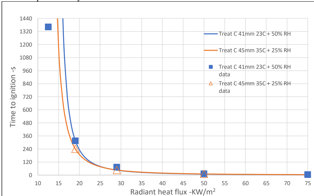
Figure 16 Plots of time to ignition for Radiata Pine with preservative treatment C(H4) based on Janssens method
