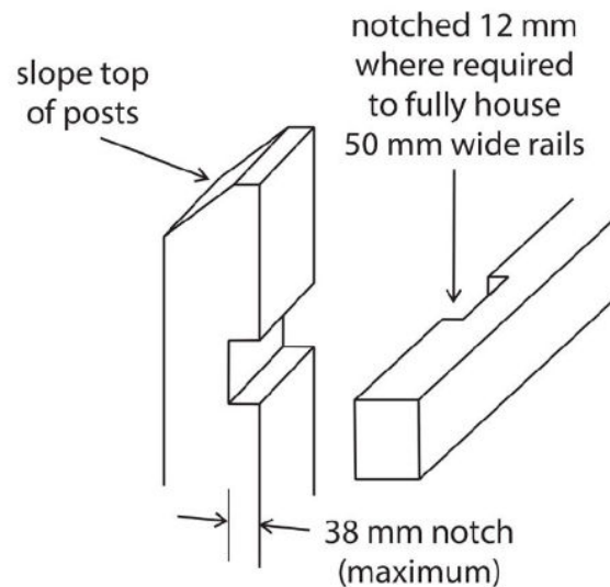
Figure 7 Notched joint from Timber Queensland technical data sheet 20 residential fences.
