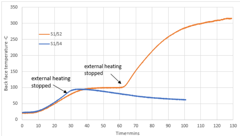
Figure 25 Rear face temperature for 45mm thick treated radiata pine subjected to an irradiance of 12.5\text{kW/m}^2 - blue plots show specimen with heating terminated 5 minutes after flaming ignition (total exposure 27.75mins); Brown plots show specimen that underwent smouldering ignition only with heating continued for total exposure of 63 minutes
