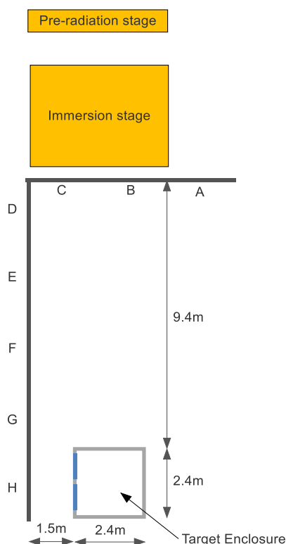
Figure 4 Test Configuration used for bushfire simulation testing derived from the description provided in (Leonard, Blanchi et al. 2006)
