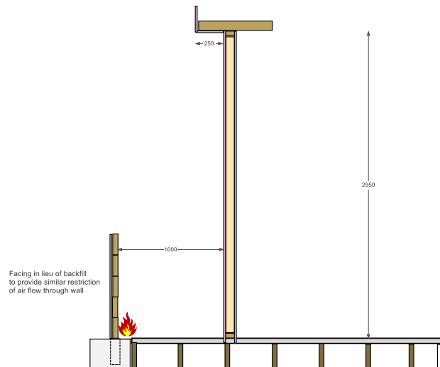
Figure 24 Section AA Garden bed retained above path with wall facing reference building - radiant heat perpendicular to face of the sleeper wall
