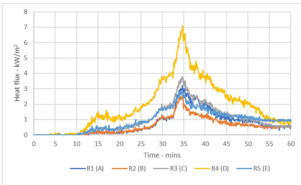
Figure 64 Ember test 1 Heat flux measured on west face of structure
