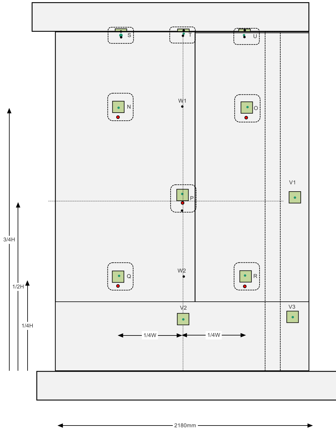
Figure 27 Elevation of north wall showing instrumentation of building perpendicular to the simulated fire source
