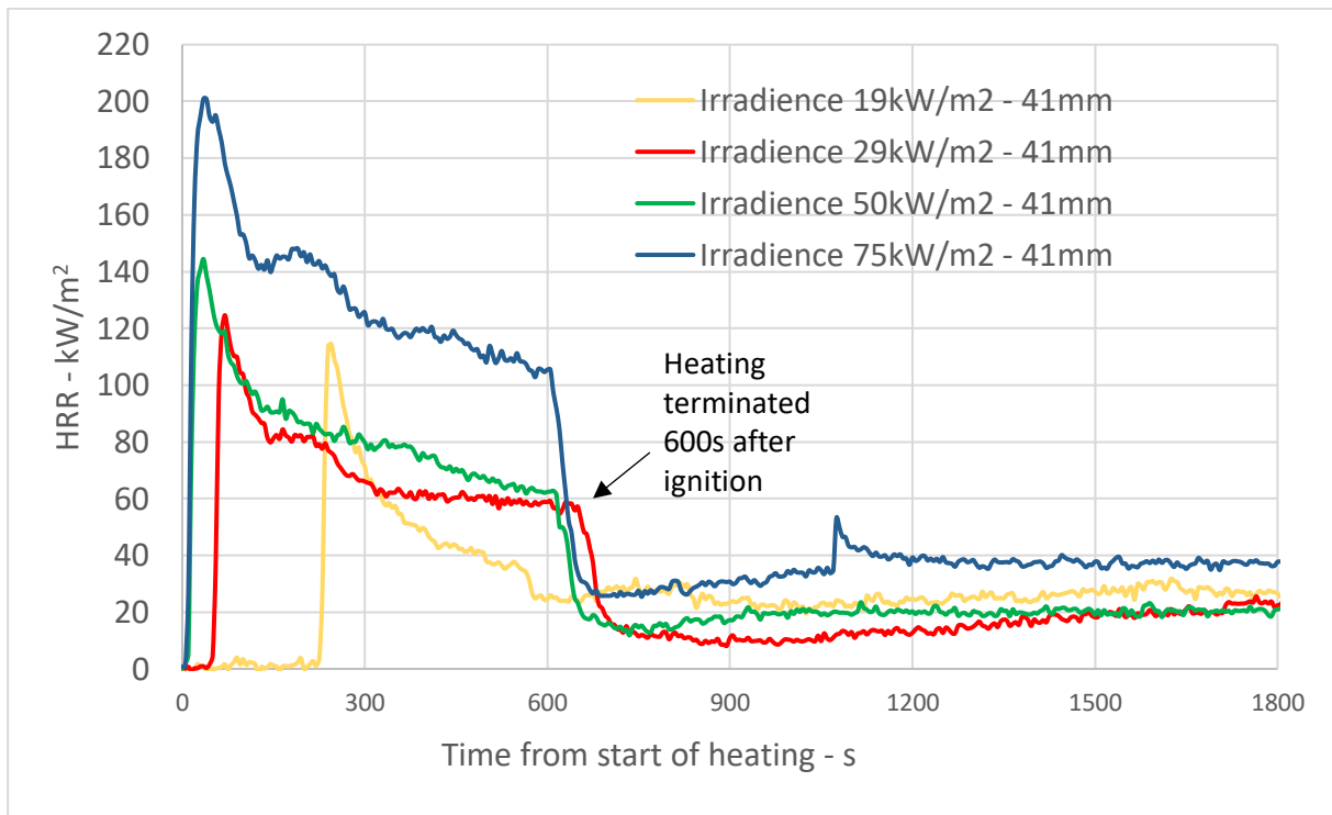
Figure 20 HRR from fire cone calorimeter tests on radiata pine, nominally 41mm thick with preservative treatment C at varying irradiances for a heating duration of 600s after ignition – specimens conditioned at 23°C and 50% relative humidity.
