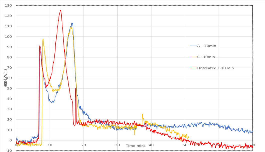
Figure 7 Heat Release Rate for 12mm palings with treatments A and C and untreated exposed to an irradiance of 19\text{kW/m}^2 before ignition and a further 10 minutes
