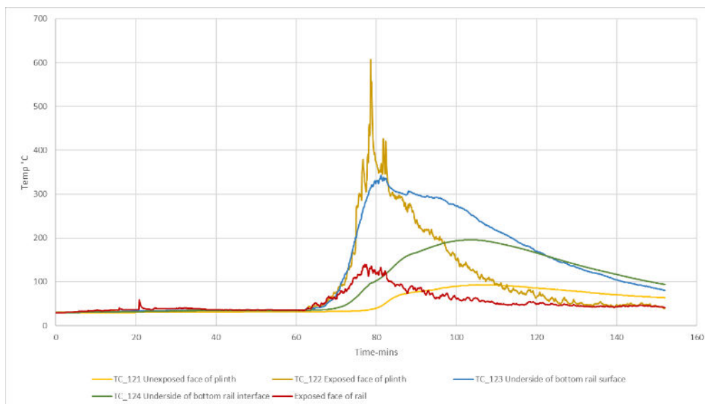
Figure 78 Temperatures measured at base of fence 100mm from east face of corner post
