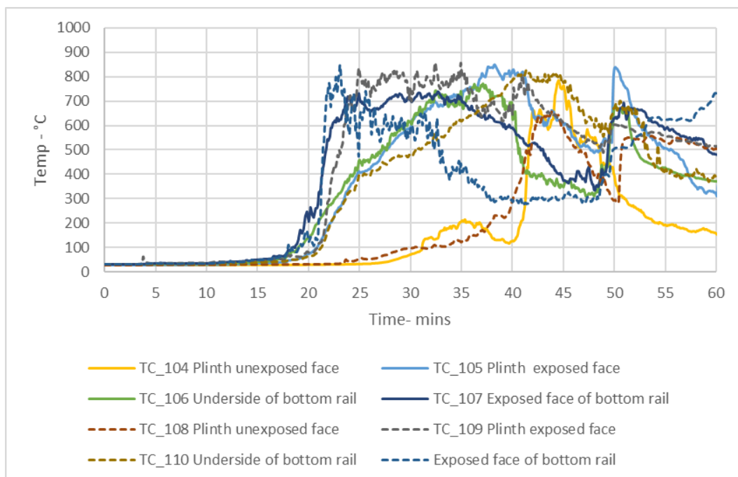
Figure 61 Plinth temperatures at a height of 25mm and bottom rail temperatures 100mm away from corner post; Solid lines are south of the corner post and dashed lines are east of the corner post
