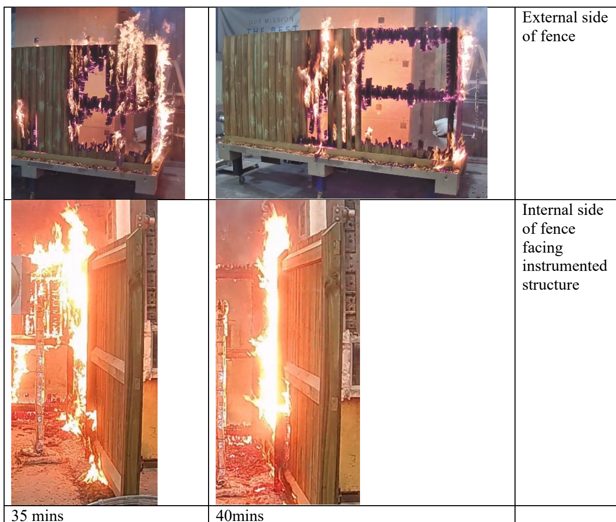
Figure 67 Fence at times corresponding to peak heat fluxes on simulated building.
