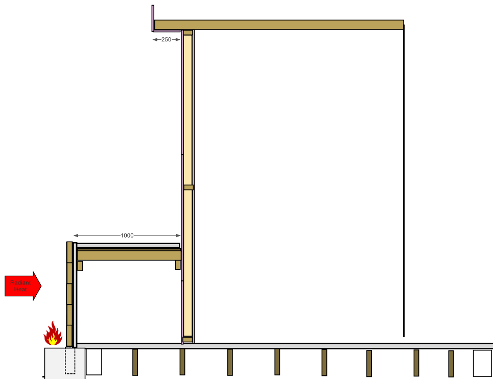
Figure 21 Section BB Retaining wall below house level 1 m in front of façade facing bushfire
