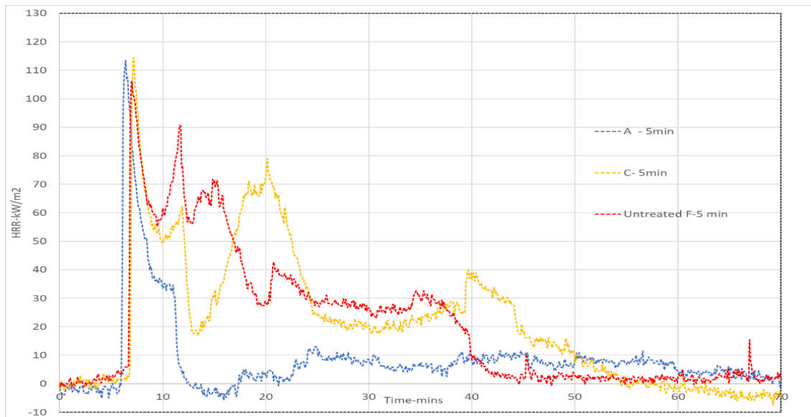
Figure 9 Heat Release Rate for 12mm palings with treatments A and C and untreated exposed to an irradiance of 19kW/m 2 before ignition and a further 5 minutes
