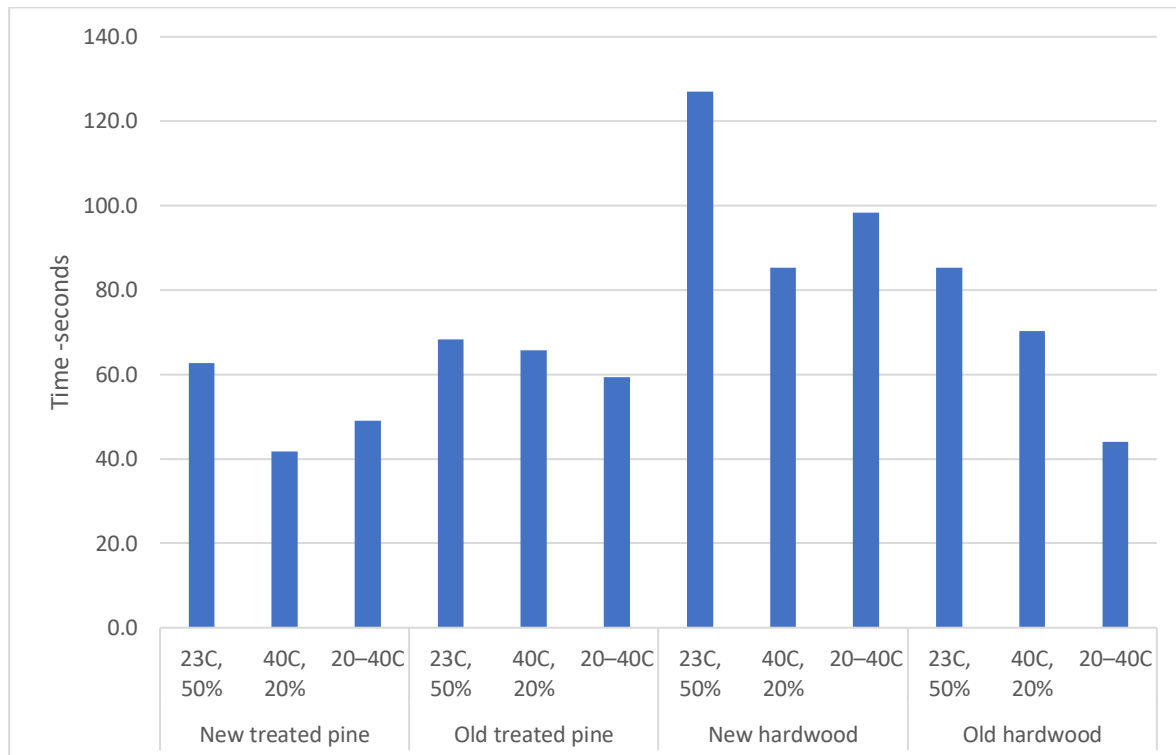
Figure 2 Mean time to ignition for samples of timber palings - derived from data presented in (Leonard, Blanchi et al. 2006)
