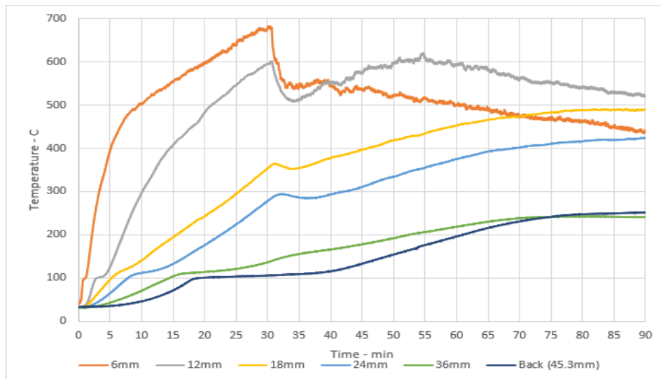
Figure 27 Internal temperatures for 45mm thick treated radiata pine subjected to an irradiance of 29\text{kW/m}^2 for 30 minutes after ignition and conditioning at 30^\circ\text{C}/25\% r.h.
