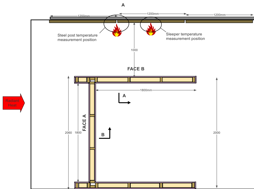
Figure 23 Garden bed retained above path with wall facing reference building - radiant heat perpendicular to face of sleeper wall,
