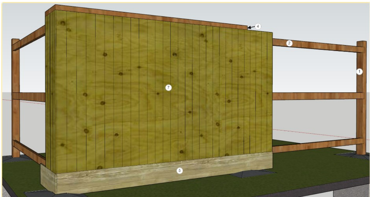
Figure 6 Paling fence system with ember shedding and timber plinth viewed from predominant vegetation side.
