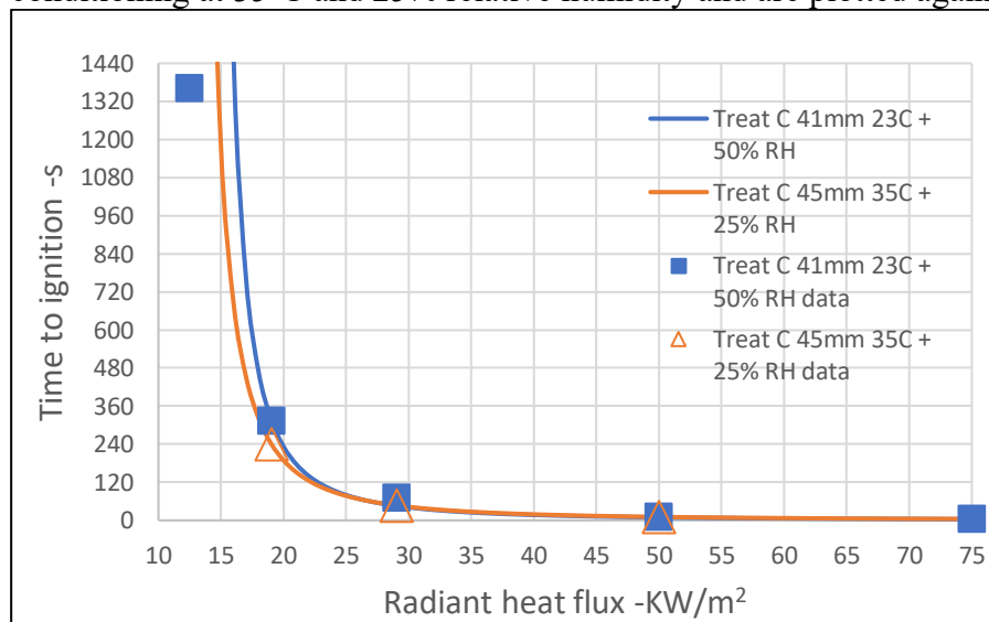
Figure 29 Plots of time to ignition for Radiata Pine with preservative treatment C(H4) based on Janssens method
