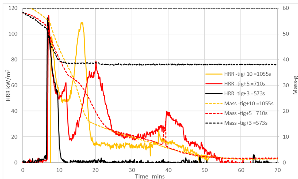
Figure 22 HHR and specimen mass for 12mm thick treated radiata pine subjected to an irradiance of 19\text{kW/m}^2 - black plots show specimen with heating terminated 3 minutes after flaming ignition (total exposure 573s) which self-extinguished when heat source removed; Red and yellow plots show specimens with longer exposures that continued smouldering combustion when heating continued.
