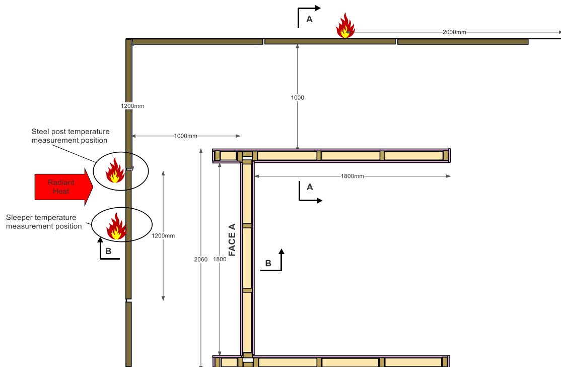
Figure 20 Sleeper wall below house level and 1 m in front of the house façade facing bushfire front.
