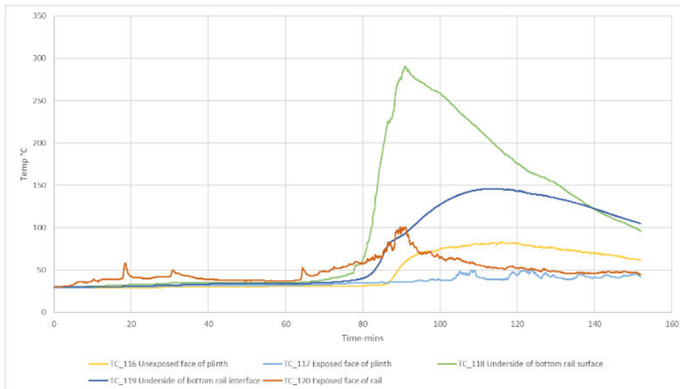
Figure 77 Temperatures measured at base of fence 500mm from south face of corner post
