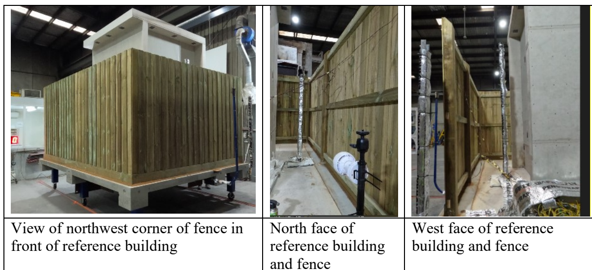
Figure 37 Fence and Reference building before test
