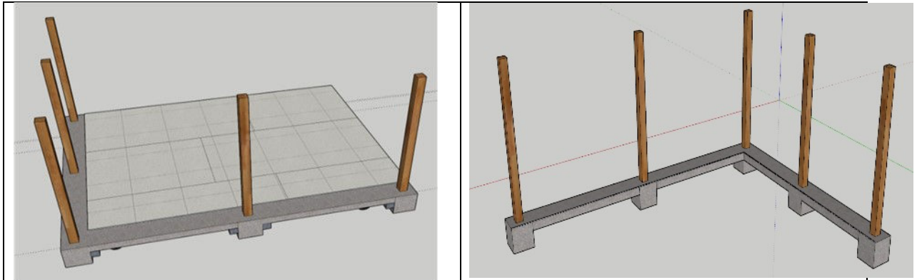
Figure 13 Schematic of test platform and pre-prepared footing assembly prior to mounting on platform
