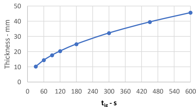
Figure 13 Bounding condition for thermally thick materials based on thickness and time to ignition
