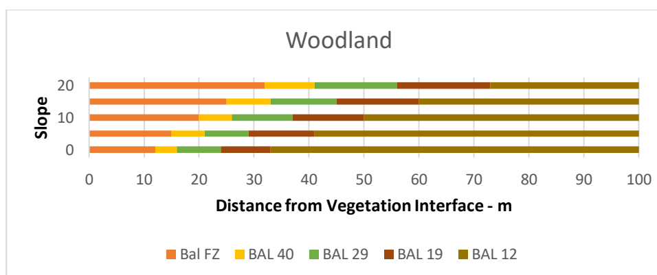
Figure 5 AS 3959 2009 BAL Levels v Distance from Woodland for varying Downslopes for an FFDI of 100 using the Simple Method Tabulated Values
