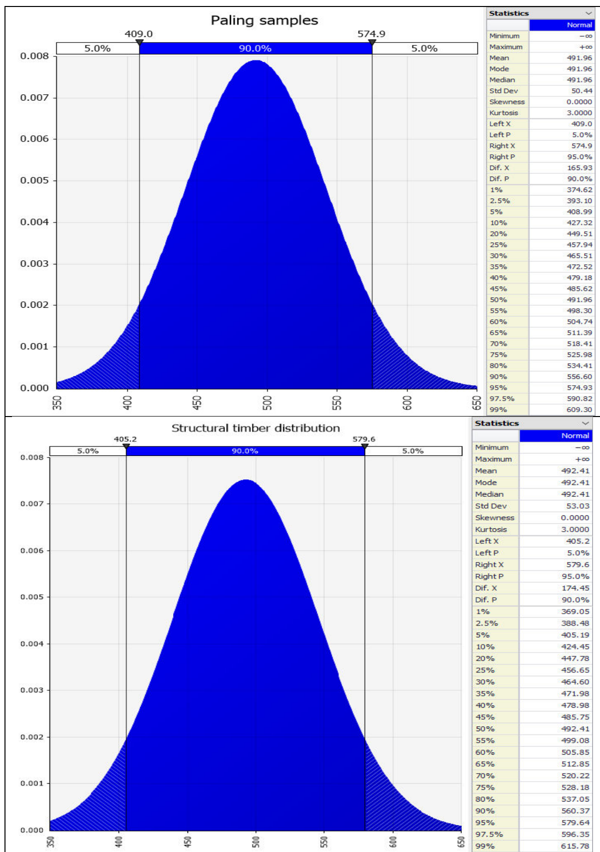
Figure 2 Distribution of densities for samples of Radiata Pine subjected to Cone calorimeter tests
