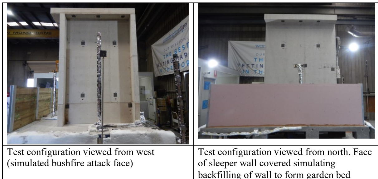
Figure 22 Garden bed configuration with sleepers facing the reference building
