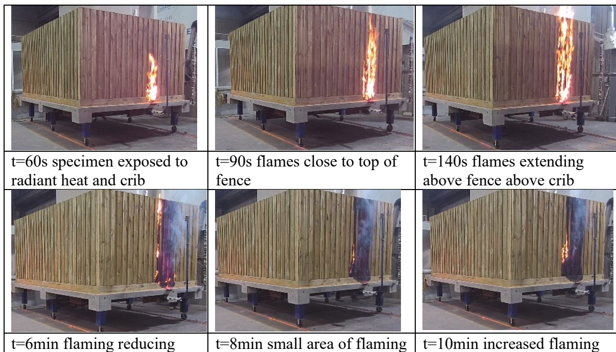
Figure 38 Fire initiation and spread under AS 1630.8.1 BAL 12.8.1 heating profile
