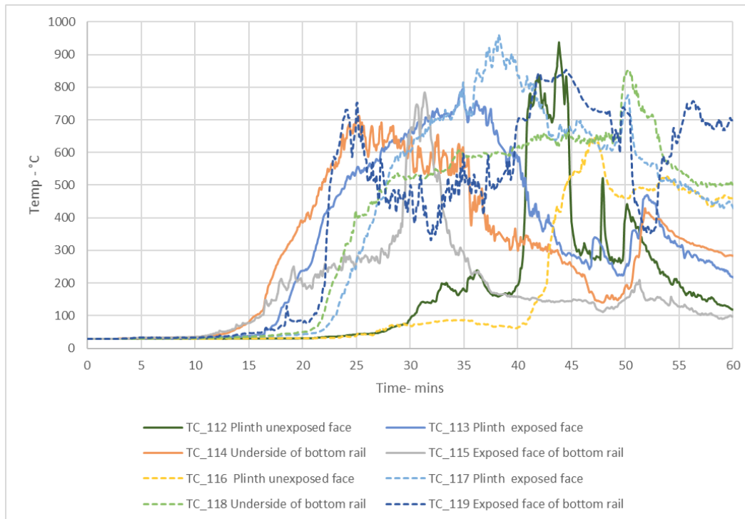
Figure 62 Plinth temperatures at a height of 25mm and bottom rail temperatures 500mm away from corner post; Solid lines are south of the corner post and dashed lines are east of the corner post
