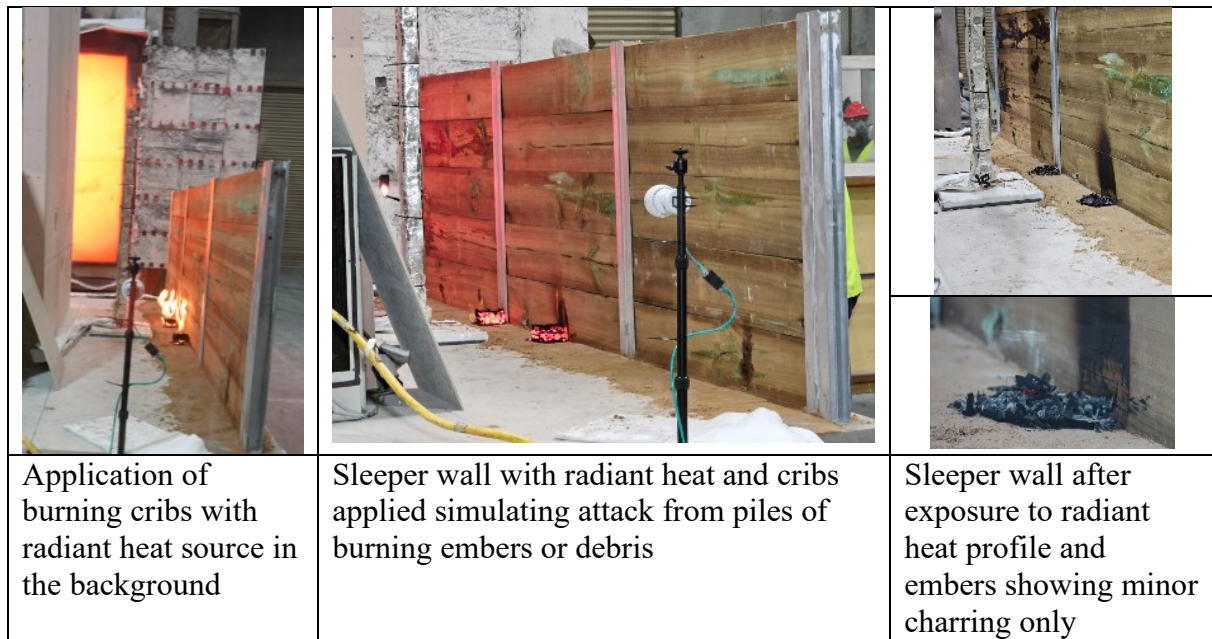
Figure 46 Crib tests applied to sleeper wall.
