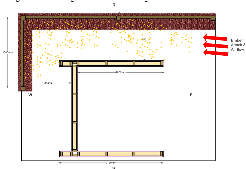
Figure 54 General Test configuration
