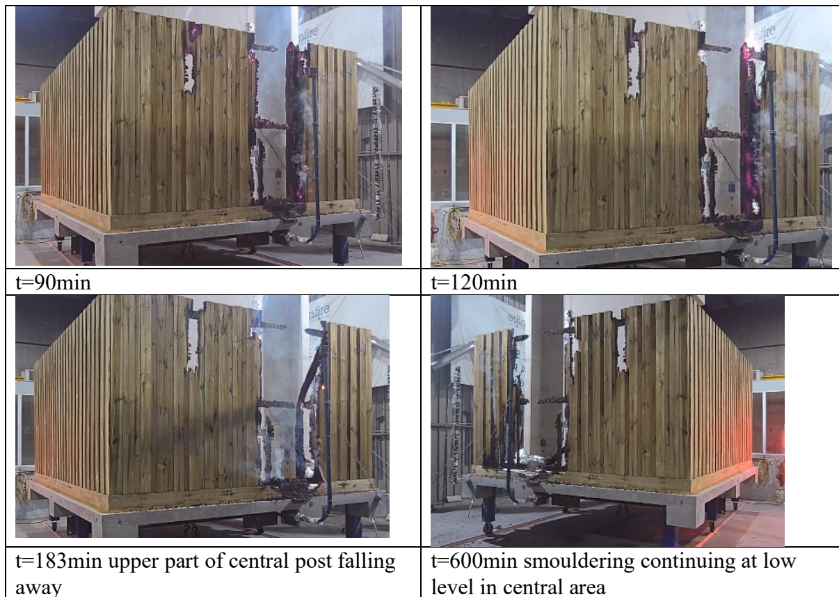
Figure 40 Continuing low level smouldering combustion in central area.
