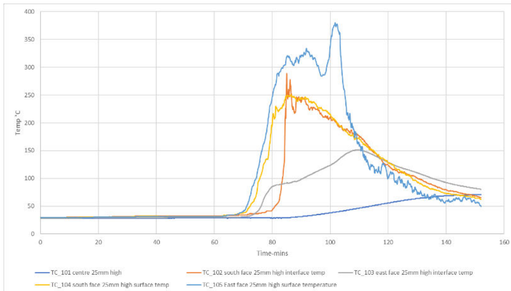
Figure 74 Corner post temperatures for ember test 2: Lapped paling fence with ground level protection
