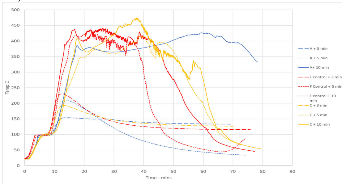
Figure 10 Temperature of back face of 12mm palings with treatments A and C and untreated, exposed to an irradiance of 19kW/m 2 before ignition and for 3, 5 and 10 minutes after ignition.
