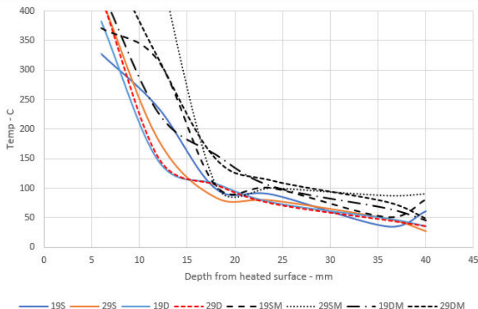
Figure 28 Temperature profiles at termination of heating for specimens subjected to irradiances of 19 and 29\text{kW/m}^2 . The suffix S is applied to specimens conditioned at 23^\circ\text{C} and 50% r.h. and D to specimens conditioned at 35^\circ\text{C} and 25% r.h. Suffix M is applied to marginal cases where there had been substantial smouldering combustion, but late self-extinguishment occurred.
