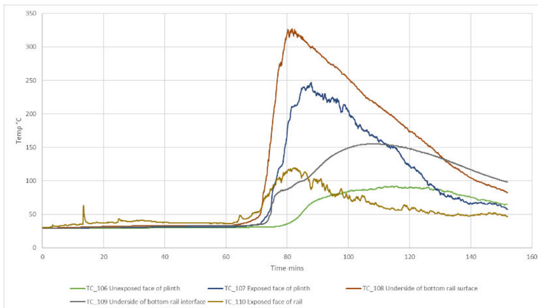
Figure 75 Temperatures measured at base of fence 100mm from south face of corner post
