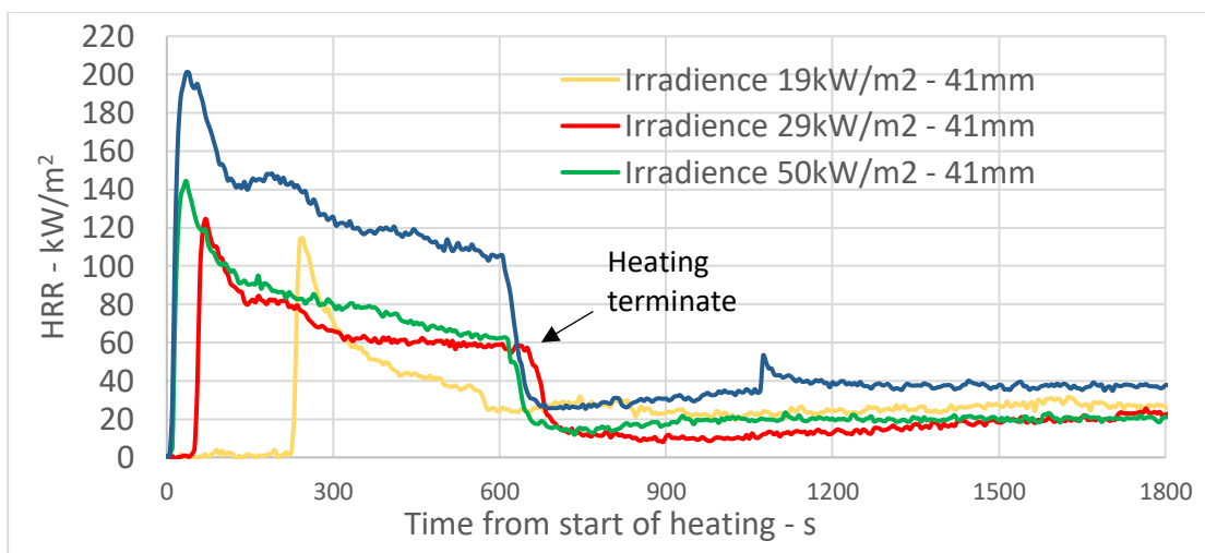
Figure 30 HRR from fire cone calorimeter tests on radiata pine, nominally 41mm thick with preservative treatment C at varying irradiances for a heating duration of 600s after ignition – specimens conditioned at 23°C and 50% relative humidity.
