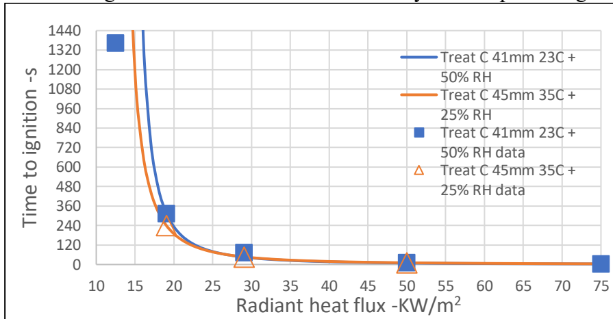
Figure 10 Plots of time to ignition for Radiata Pine with preservative treatment C(H4) based on Janssens method
