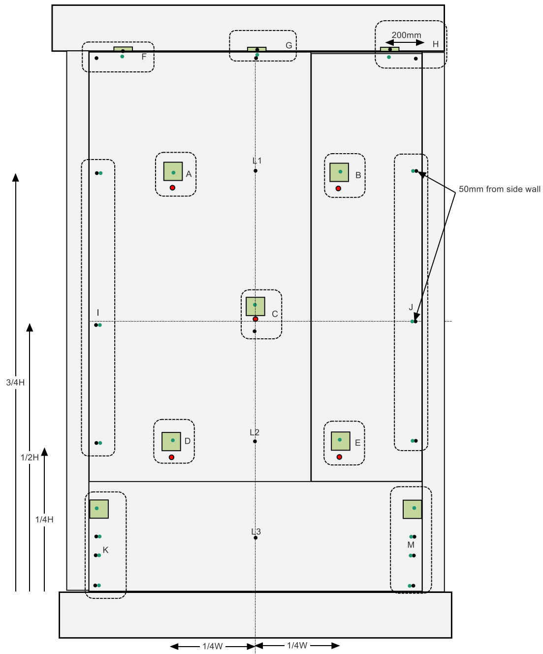
Figure 25 Elevation of west wall of reference building showing instrumentation of building facing the simulated fire source.
