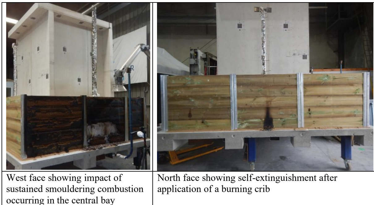
Figure 51 Sleeper walls approximately 19 hours after start of test
