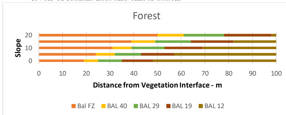
Figure 4 AS 3959 2009 BAL Levels v Distance from Forest for varying Downslopes for an FFDI of 100 using the Simple Method Tabulated Values
