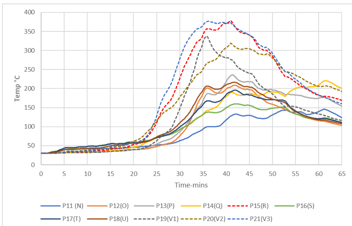
Figure 65 Plate thermometer measurements on the north face of simulated building
