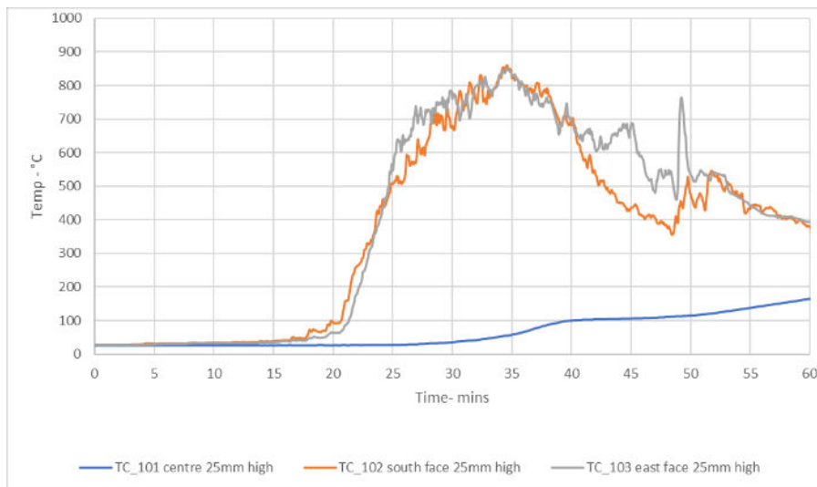
Figure 60 Corner post temperatures for ember test 1: Lapped paling fence with mulch at base of exposed to ember attack with applied airflow
