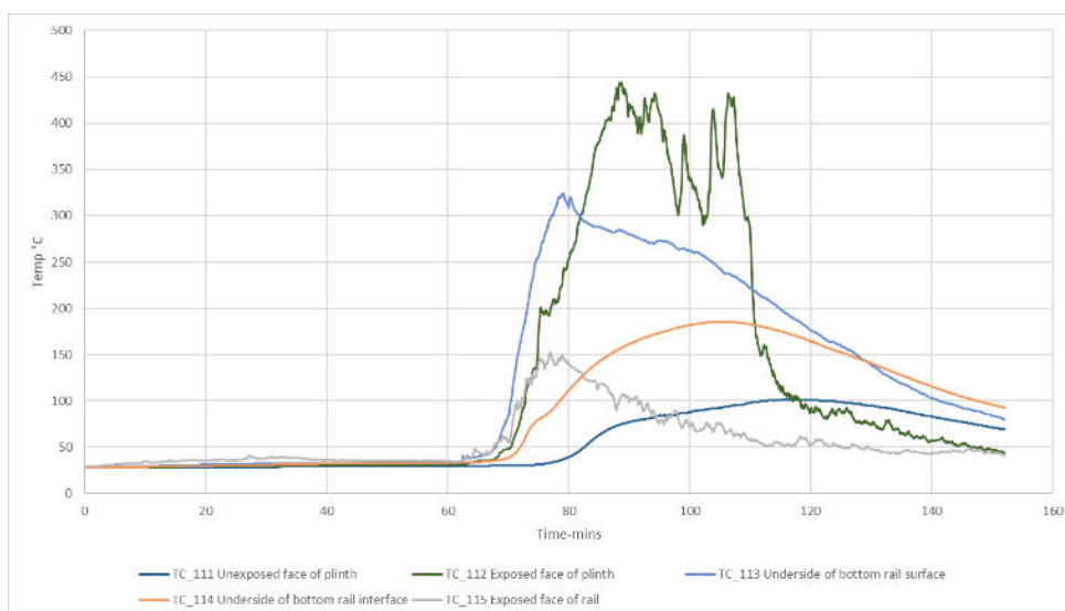
Figure 76 Temperatures measured at base of fence 100mm from east face of corner post
