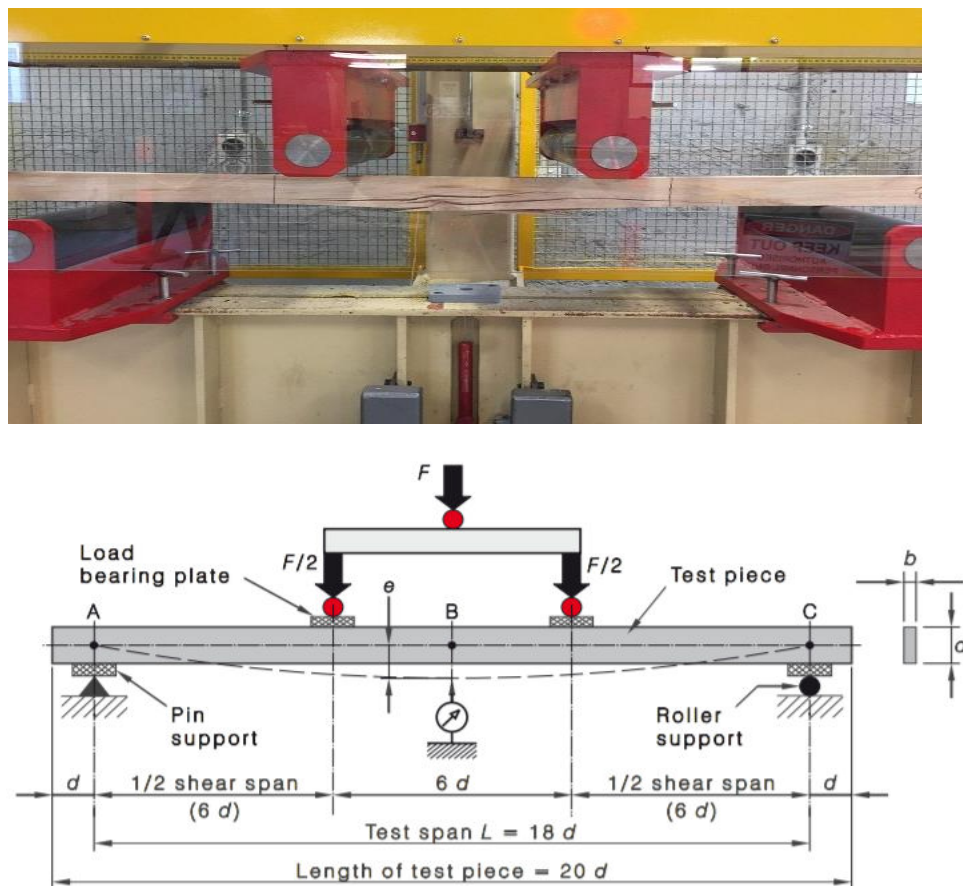
Figure 2. Static four-point bending test
