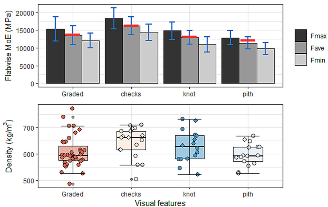
Fig. 7. Static flatwise MoE mean values (filled bars) and standard deviation among visual features. The horizontal short lines (blue) are standard deviation bars. The horizontal lines (red) are static edgewise MoE mean values. Density (MC being adjusted to 12%) among visual features. (For interpretation of the references to colour in this figure legend, the reader is referred to the web version of this article.)
