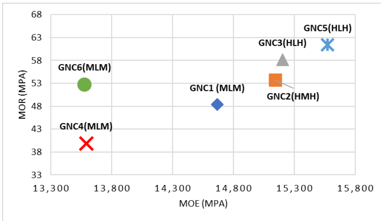
Figure 5 Static MoE and MoR of 6 glulam samples
