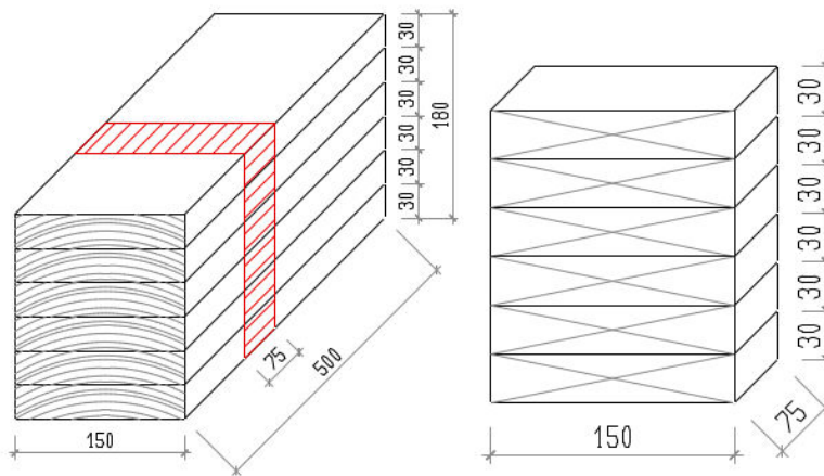
Figure 12. Laminated beam and specimen (red and right) as required by EN 302-2
