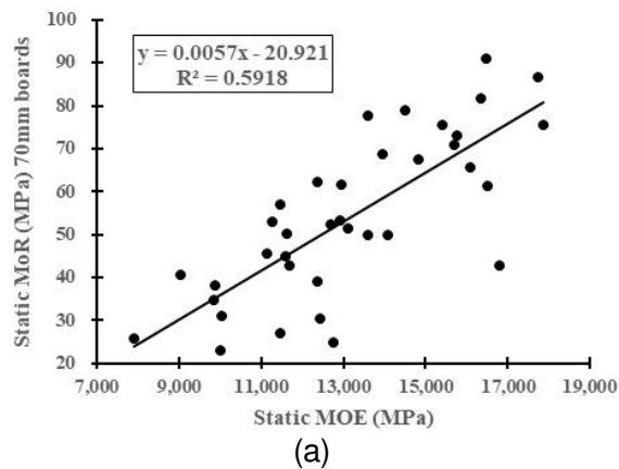
Figure 5 Relationship between static MOR and static MOE(a) and between static MOR and AWW (b)
