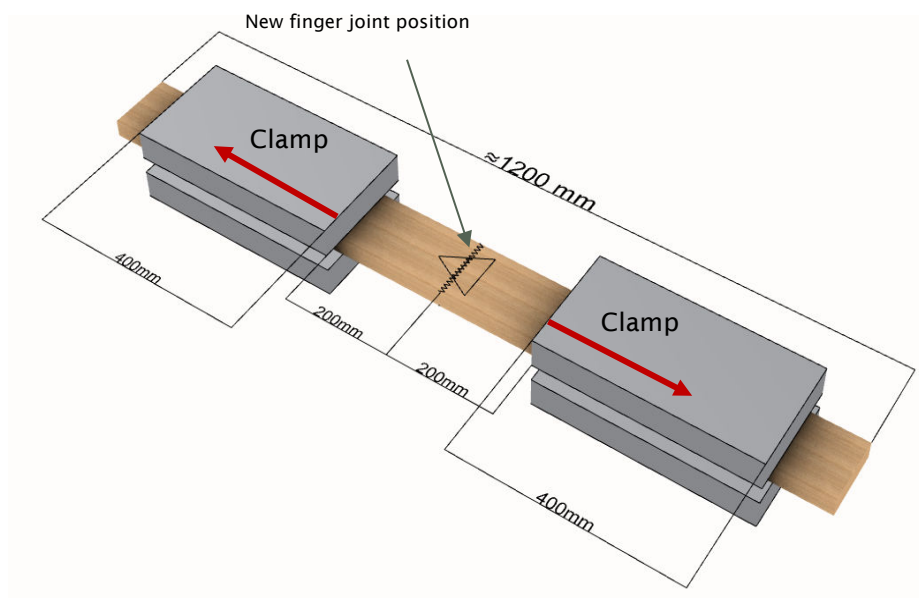
Figure..1: simplified setup of the tension test with the position of the new finger joint and the clamps.
