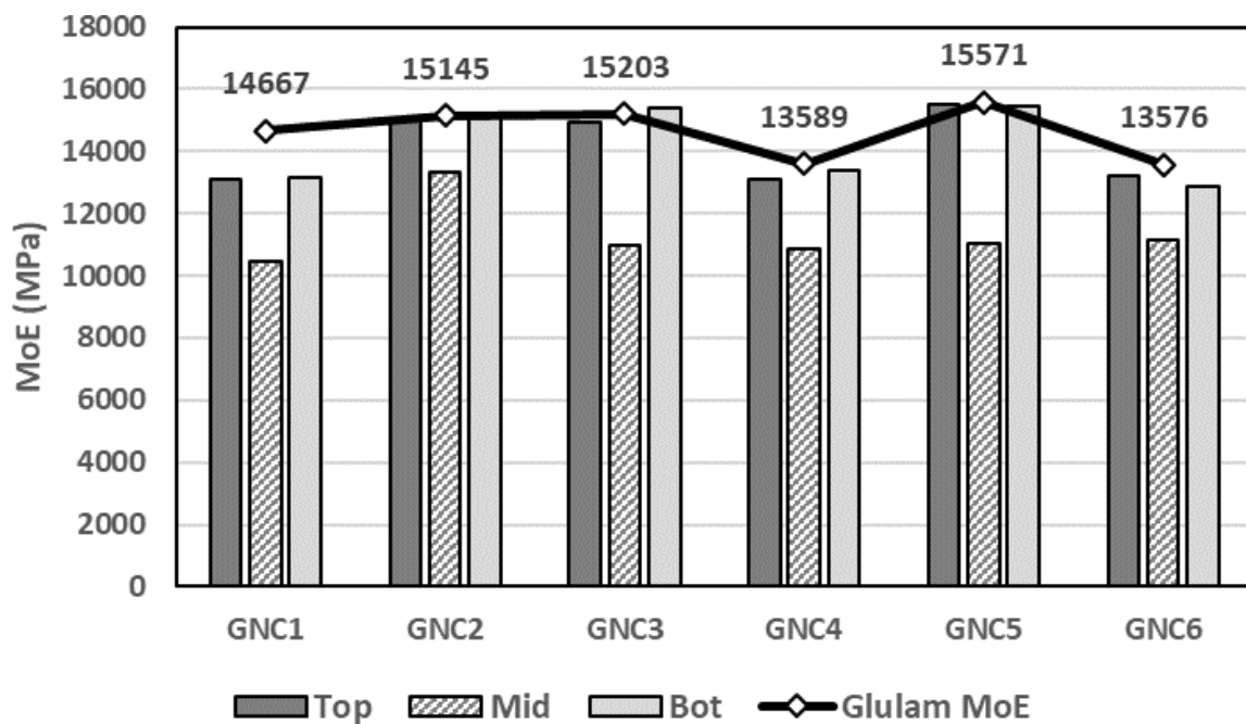
Figure 3: The result of 6 glulam elements and dynamic MoE of the laminations
