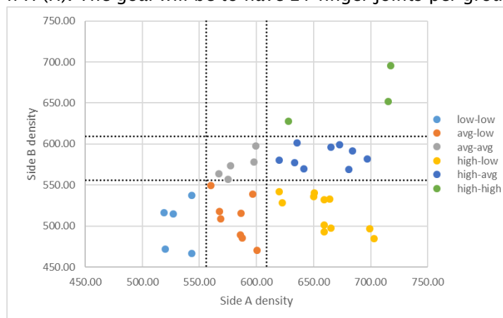
Figure 6: Density class of each new finger joint made at n'H shown based on the density of the two connecting members. The dashed lines represent the lower and upper limit of the average density (556-609 kg/m 3 ).
