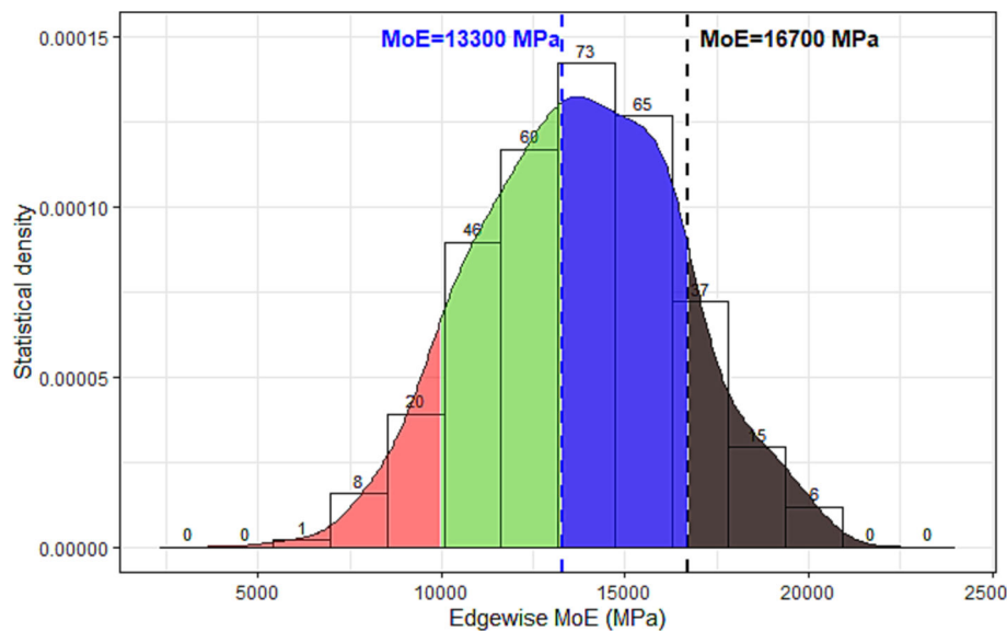
Fig. 4. Static edgewise MoE distribution (n = 331).
