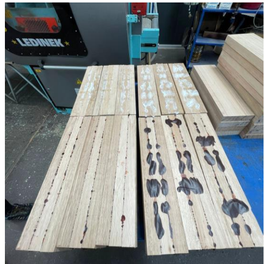
Figure 4. GLT showing different glue types.
