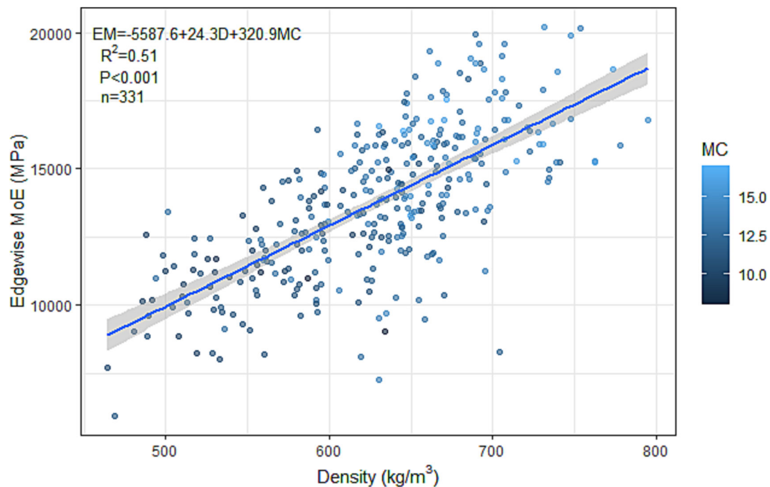
Fig. 6. Relationship between density and static edgewise MoE (filled circles). The straight line is static edgewise MoE estimated by D and MC. And the grey region depicts the 95% confidence interval for the mean.
