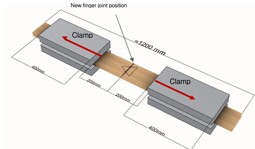
Figure 9. simplified setup of the tension test with the position of the new finger joint and the clamps
