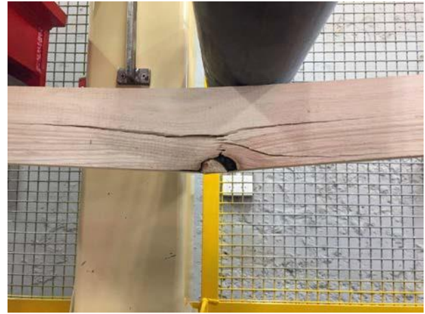
Figure 2 Failure mode of the E. nitens boards in bending
