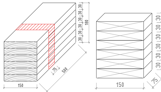
Figure 10 : Laminated beam and specimen (red and right) as requested by EN 302-2
