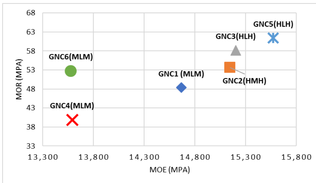
Figure 7. Static MoE and MoR of 6 glulam samples
