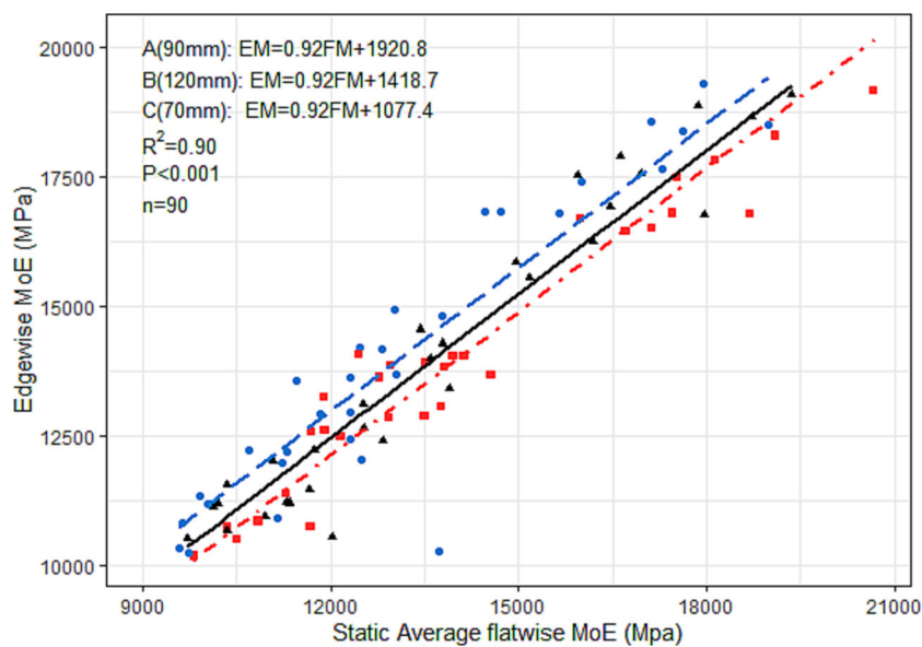
Fig. 9. Relationship between static edgewise MoE and static average flatwise MoE (filled shapes). Straight lines are static edgewise MoE estimated by static average flatwise MoE for different width groups of boards.
