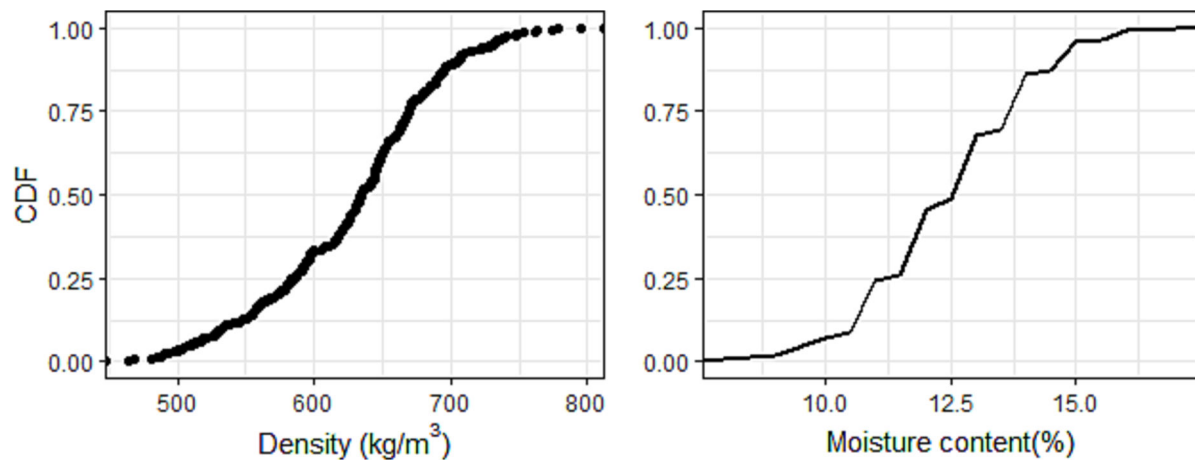
Fig. 1. Cumulative distribution of density and moisture content.
