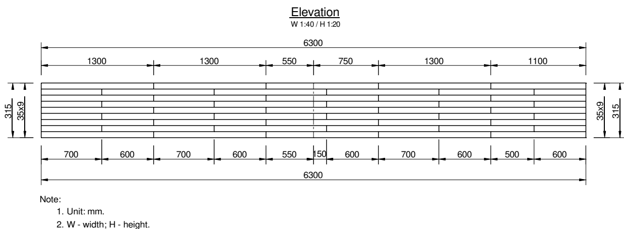
Figure 1: Elevation view of the tested beams
