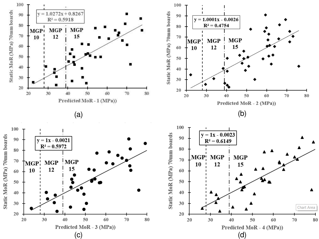
Figure 6 Predicted MOR values using the linear regression equations
