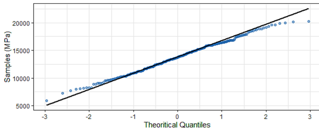
Fig. 5. The quantile-quantile (Q-Q) plots for the edgewise MoE (n = 331).
