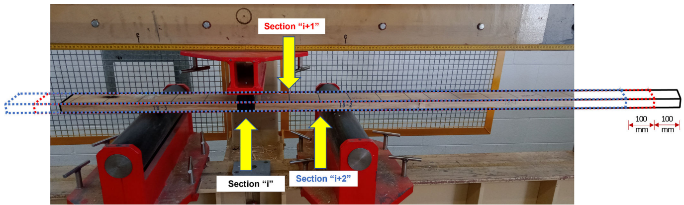
Fig. 3. Three points bending tests setup (flatwise).
