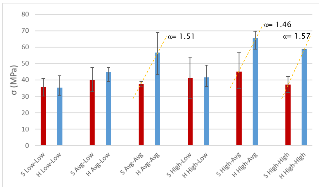
Figure 7: Average strength by class and process
