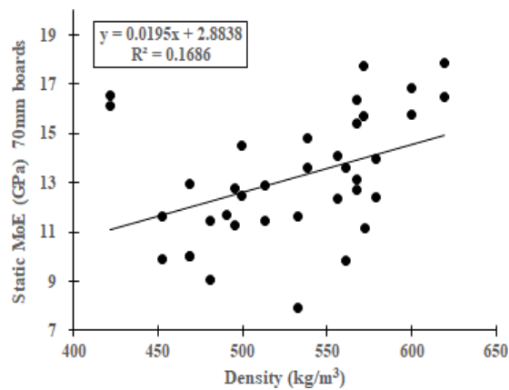
Figure A1 Correlation between MOE and density
