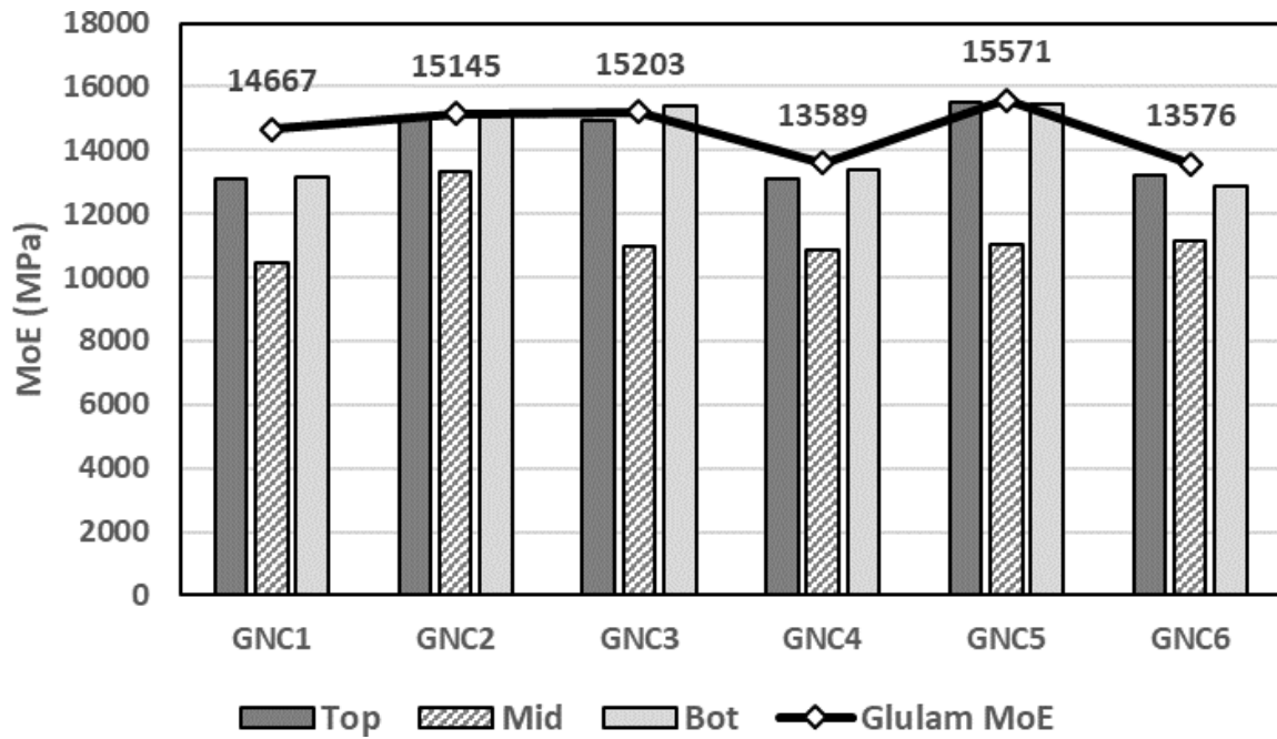
Figure 6. The result of six glulam elements and dynamic MoE of the laminations
