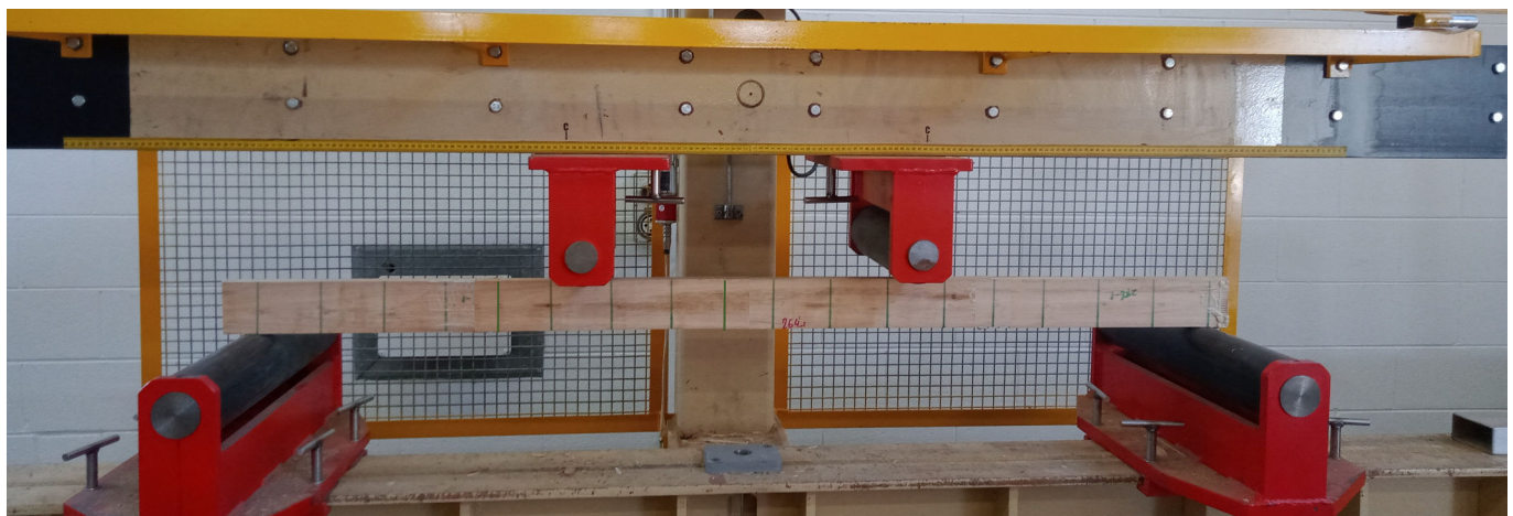
Fig. 2. Four points bending tests setup (edgewise).
