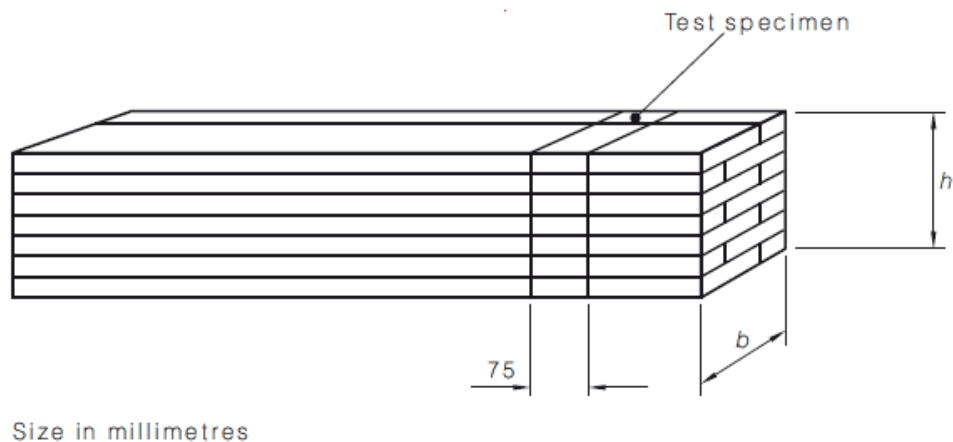
FIGURE C1 TEST SPECIMEN CUT FROM A GLULAM MEMBER
