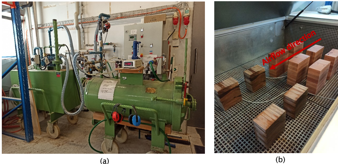
Figure 11 : Devices used in delamination test; a) Autoclave, b) Air dryer with controlled humidity and airflow speed.
