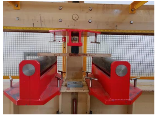
Figure 10. Three point bending test on finger joint samples at CSAW.
