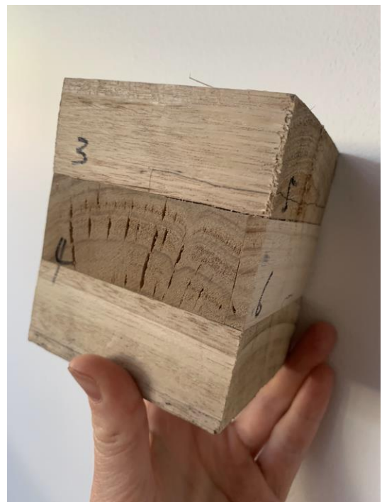
Figure 11. CLT block showing signs of delamination
