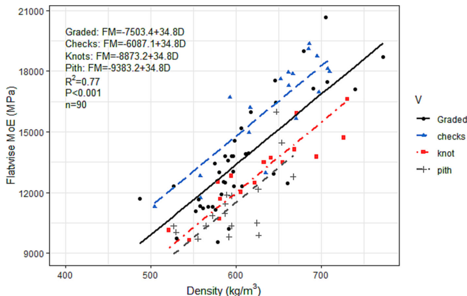
Fig. 8. Relationship between density and static average flatwise MoE (filled shapes). Straight lines are static flatwise MoE estimated by density for different visual features groups of boards.
