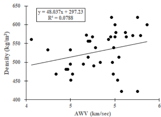
Figure A2 Correlation between density and AWW
