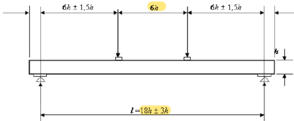
Figure 17 — Test arrangement for measuring bending strength
