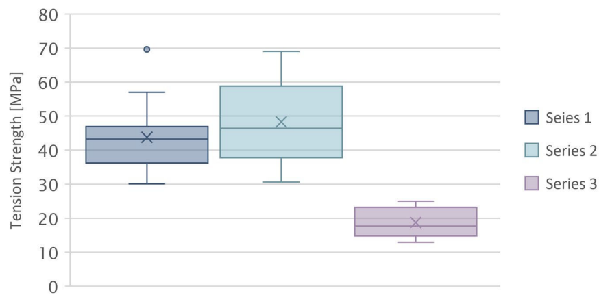
Figure 4: Boxplot of the different series where the x represents the average and the box the quartile and the line in the box the median.
