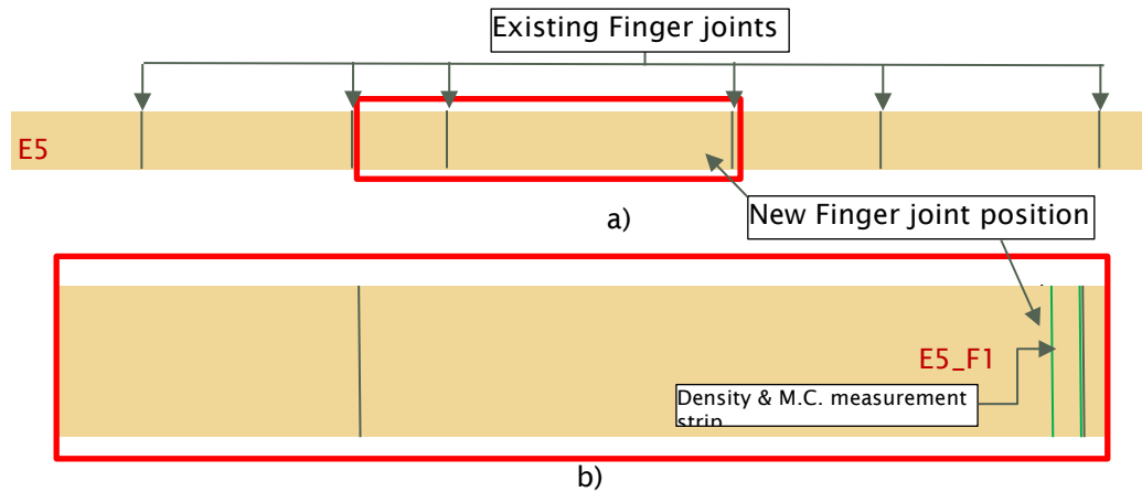
Figure. 2: a) The original length (=3m) of the received board, the position of the existing finger joints, and the possible position of one side of a new finger joint. b) The part (min 1 m) of the original board suitable for one side of a finger joint and the position of the density and M.C. measurement strip.
