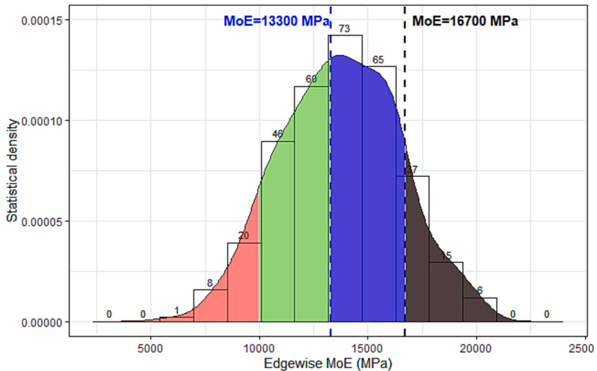
Fig. 4 Static edgewise MoE distribution (n = 331)
