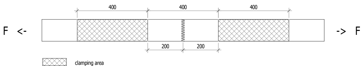
Figure 1: schematic sketch of the test setup
