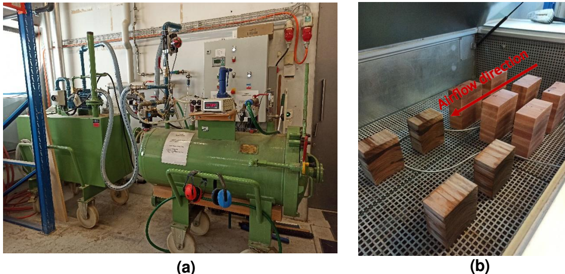
Figure 13. Devices used in delamination test, (a) Autoclave, Air dryer with controlled humidity and airflow speed (b)
