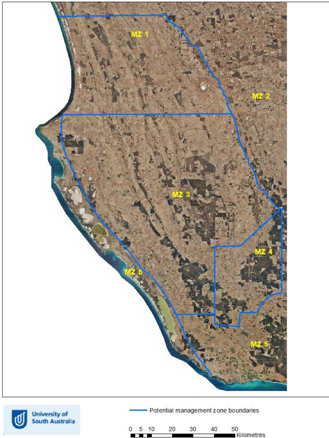
Figure 6: Potential Lower Limestone Coast Management Zones based on unconfined aquifer thickness and structural elements
