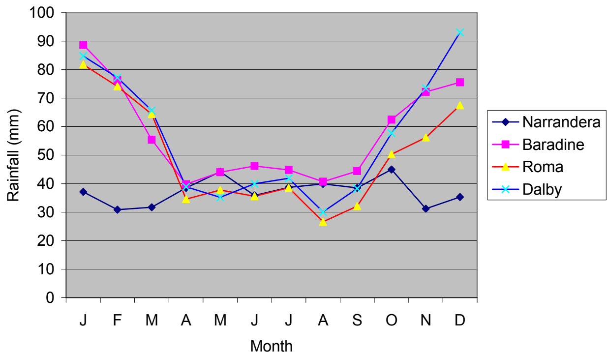
Figure 1. Mean annual rainfall at Narandera, Baradine, Roma and Dalby (from Bureau of Meteorology – Climate Averages )
