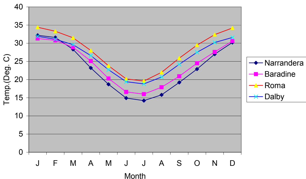
Figure 2. Mean daily maximum temperature for Narrandera, Baradine, Roma and Dalby (from Bureau of Meteorology – Climate Averages).
